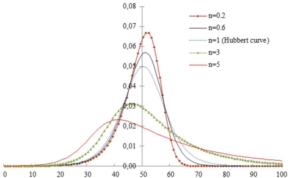
Figure 4. Production behaviours under different curve shape.
