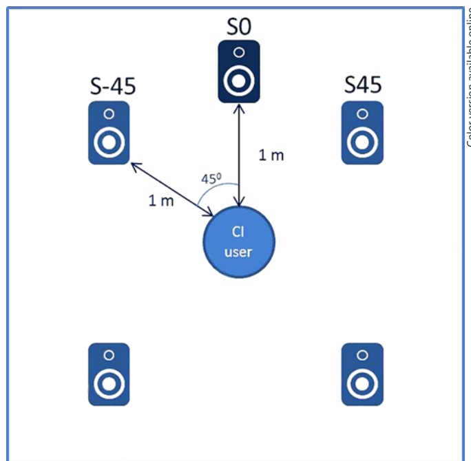
Fig. 2. A schematic representation of the test environment. The cochlear implant (CI) user is in the middle of 5 loudspeakers, all at a distance of 1 m. The target signal is coming from S0 for the static listening condition and randomly from the loudspeaker at -45^\circ or 45^\circ for the dynamic listening condition.
