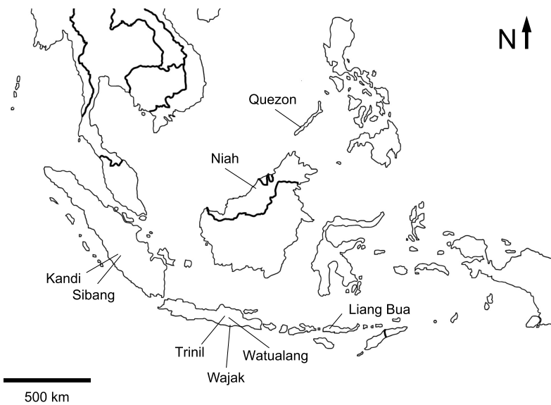
Figure 1 Map of Insular Southeast Asia indicating the location of localities with fossil bird remains.
