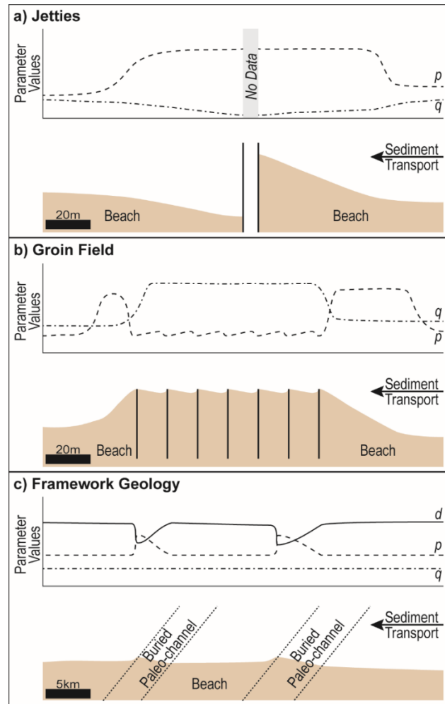
Figure 2: Sample beach-dune alongshore data series and ARFIMA model parameters ( p = \text{AR} ; d = \text{LRD} ; and q = \text{MA} ) for three coastal geomorphology scenarios. (a) Jetties trap sediment on the beach updrift side and starve the downdrift beach of sediment (see Ocean City, Maryland, USA), resulting in increased AR values on either side of the jetty. (b) Groin fields can trap sediment between the groins within the field, while starving the downdrift beach of sediment. In this case, beach volume at a particular location within the field can be modelled as the MA of adjacent beach volume measurements. Outside of the groin field, beach volume may increase/decrease, resulting in increased AR values and decreased MA values. (c) Framework geology, such as infilled paleo-channels, influences coastal geomorphology on broader spatial scales (see oblique gravel ridges in the Outer Banks, North Carolina, USA) is much more likely to appear in the LRD values. While coastal morphology at broad-scales is influenced by the entire data series, sediment transport gradients can be influenced by more localized processes, resulting in an inverted trend with the AR component. The degree to which a particular point is influenced by the entire data series at a particular scale can be modelled and plotted using the LRD parameter.
