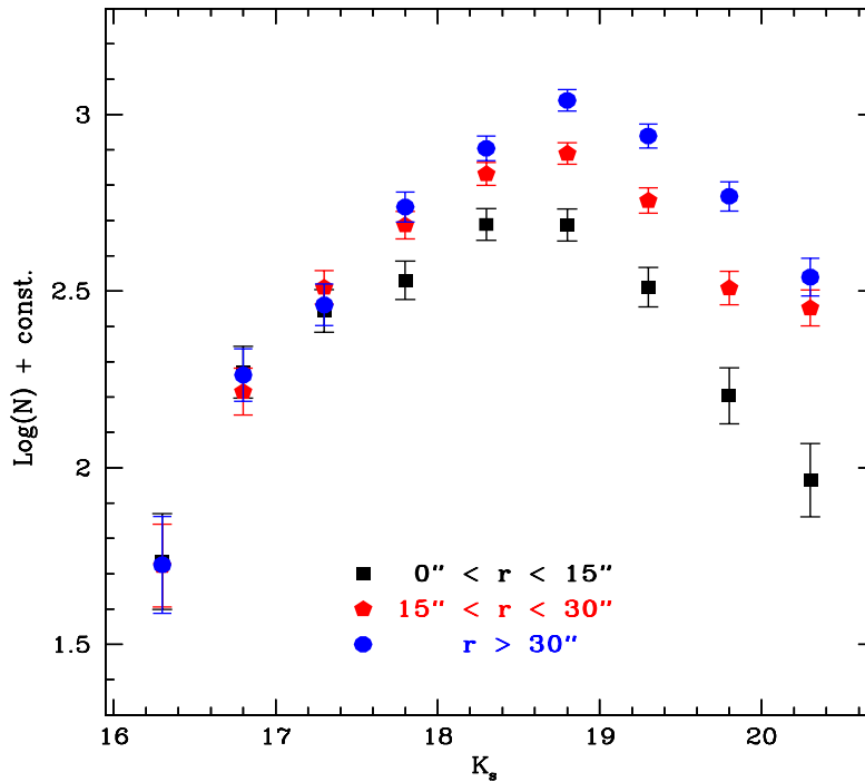
Figure 5.16: NGC 6624 completeness-corrected and field-decontaminated MS-LFs in the K_s band obtained from the GEMINI catalog in three different radial bins. The LF corresponding to the innermost radial bin is used as reference to normalize those at larger radii at the brightest bin.
