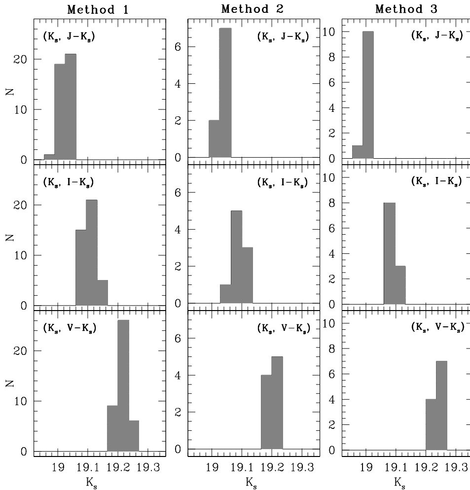
Figure 6.8: Histograms of the MS-saddle K -band magnitude measured in the (K_s, J - K_s) , (K_s, I - K_s) , and (K_s, V - K_s) CMDs (upper, middle, and bottom rows, respectively), for NGC 6624. Multiple measures of this value have been obtained in each case because the MS MRL has been determined with different methods (see Section 6.4): Method 1 - static bins (left column, providing 41 MRLs and 41 measures of the MS-saddle magnitude), Method 2 - dynamic bins (central column, 9 measures), and Method 3 - Polynomial fit (right column, 11 measures).
