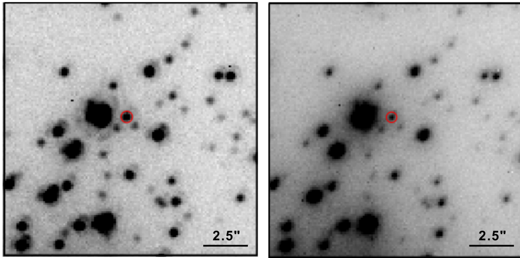
Figure 5.18: Left panel: K_s image of a region of ( 2.5'' \times 2.5'' ) of NGC 6624, centered on the position of ComStar1, marked with a red circle, as observed by the GeMS/GSAOI system. Right panel: The same, but for the J band.
