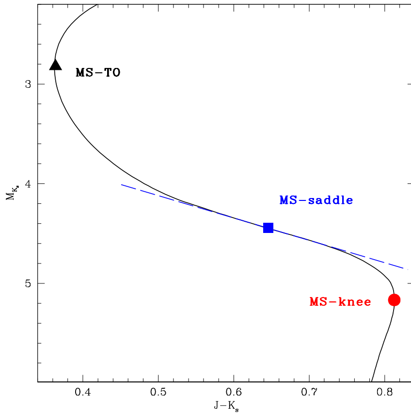
Figure 6.2: Location of the MS-TO (black triangle), MS-knee (red circle) and MS-saddle (blue square) along a 12 Gyr old isochrone extracted from the family of VandenBerg et al. (2014). The MS-knee is here defined as the reddest point along the MS MRL. The MS-saddle is the point where the MS MRL changes shape, from convex to concave, and thus shows the minimum curvature. A dashed line tangential to the isochrone is shown at the MS-saddle point to better illustrate the morphological meaning of this point.
