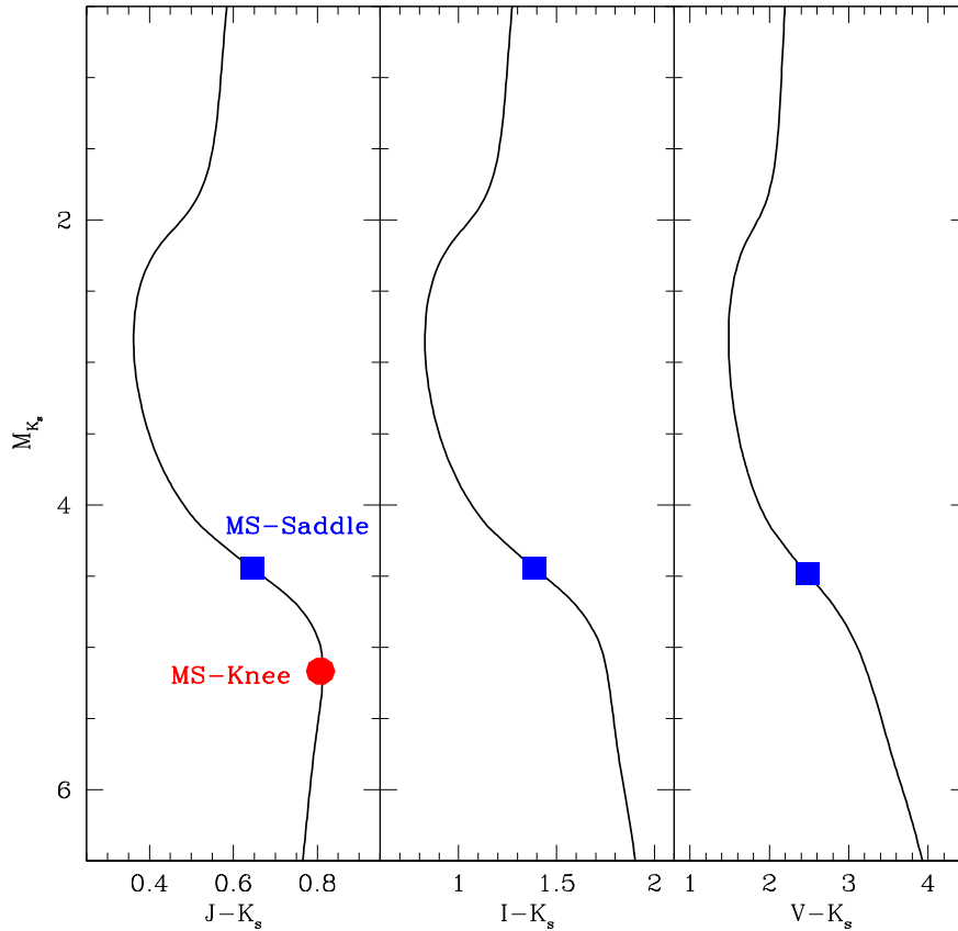
Figure 6.3: Location of the MS-knee (red circle) and MS-saddle (blue square) marked along the same isochrone plotted in Figure 6.2, but here shown in CMDs with three different colors: from left to right, (K_s, J - K_s) , (K_s, I - K_s) , and (K_s, V - K_s) . The MS-knee only occurs in the pure NIR-CMD. The MS-saddle, instead, can be defined in all the considered diagrams.
