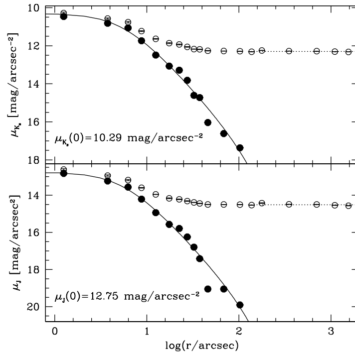
Figure 4.11: SB profiles of Liller 1 in the K_s and J bands (top and bottom panels, respectively), obtained from the 2MASS data set. Empty circles represent the observed profile, while solid ones are obtained after background subtraction (marked with a dotted line). In both panels, the solid line corresponds to the best-fit King model shown in Figure 4.10.
