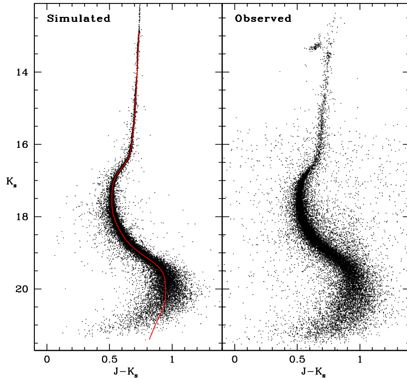
Figure 5.14: Simulated ( left panel ) and observed ( right panel ) (K_s, J - K_s) CMD of NGC 6624, for all the stars that survived the selection: -0.2 \leq \text{sharpness} \leq 0.2 . As clearly visible, the two CMDs turn out to be fully comparable, especially in the MS region (at K_s > 16 ). The red line in the left panel represents the MRL of NGC 6624 in the (K_s, J - K_s) CMD.
