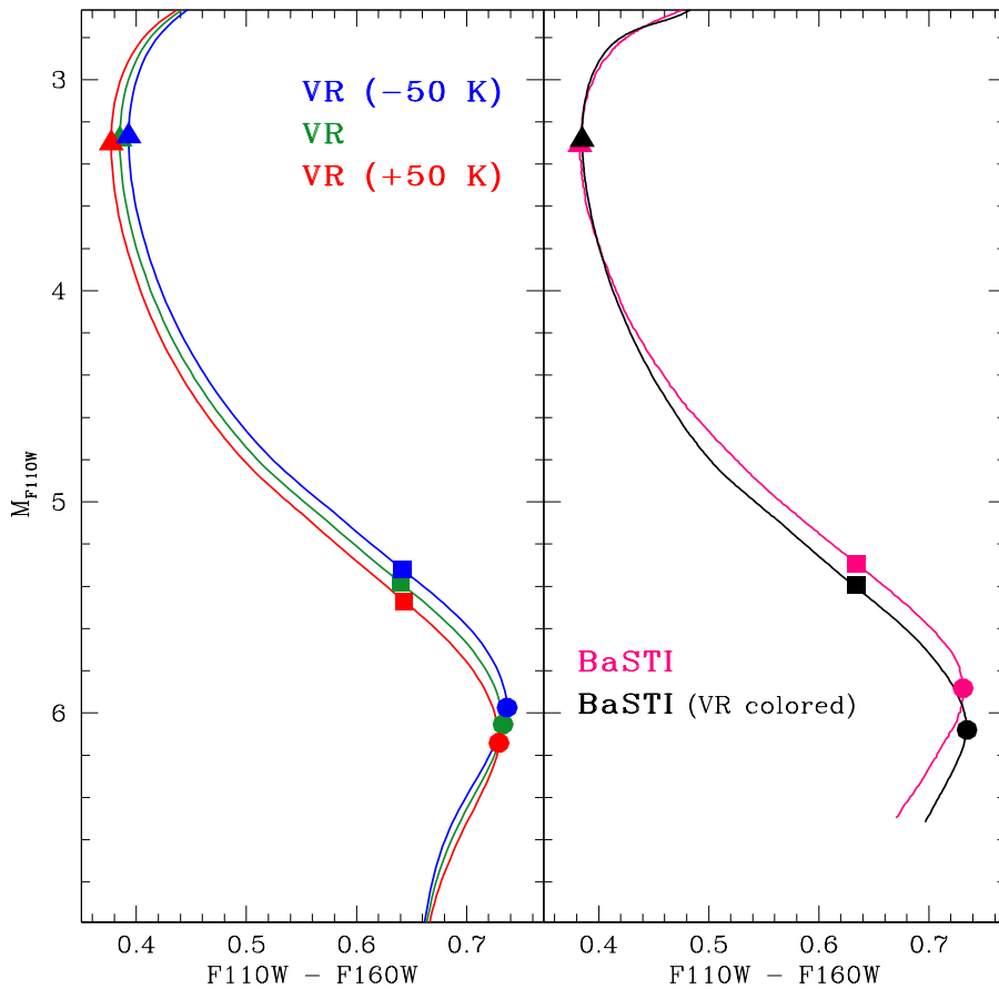
Figure 6.6: Left panel: A VR isochrone is adjusted to hotter (red line) and cooler (blue line) temperatures by 50 K with respect to the normal one (green line) and then transformed to the observed ( F110W, F110W - F160W ) plane. Right panel: In the same filter combination, a BaSTI isochrone colored using its usual BCs is shown in magenta, compared to the same isochrone colored using the Casagrande and Vandenberg (2014) BCs (in black). Triangles, squares and circles indicate the MS-TO, MS-saddle and MS-knee, respectively, in both panels.
