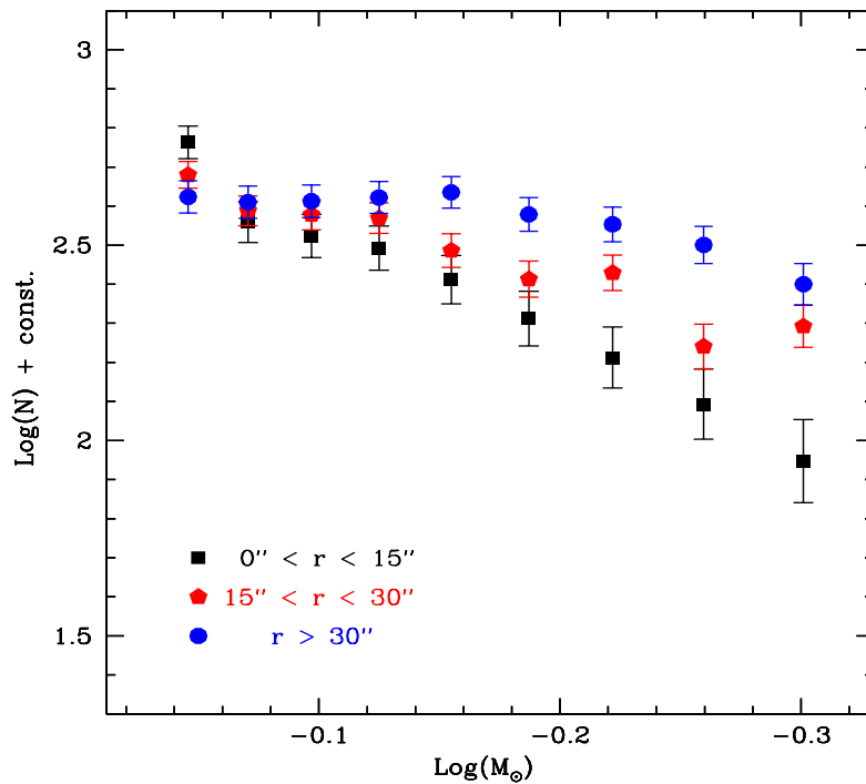
Figure 5.17: MFs derived by using a BaSTI isochrone with [\text{Fe}/\text{H}] = -0.60 and t_{\text{age}} = 12.0 Gyr (see Section 4.1). Radial bins, symbols and colors are the same as in Figure 5.16.
