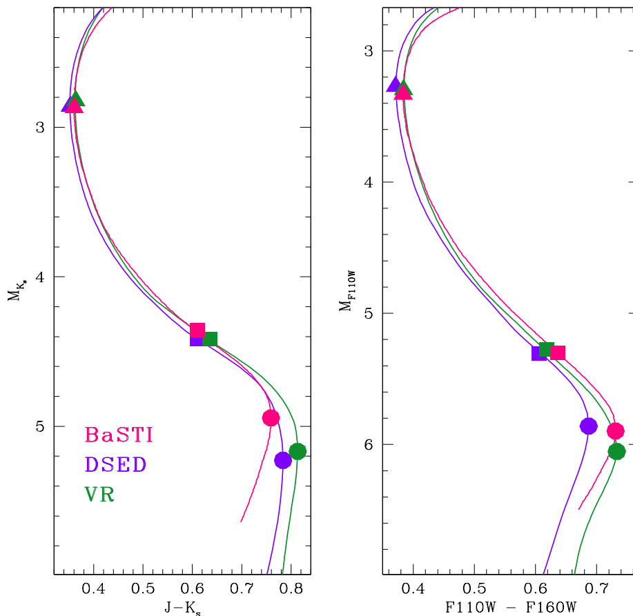
Figure 6.4: Location of the MS-TO (triangles), MS-knee (circles) and MS-saddle (squares) marked along 12 Gyr old isochrones from three different sets of theoretical models: BaSTI (magenta), DSED (purple) and VR (green) in the (K_s, J - K_s) , left panel and (F110W, F110W - F160W) , right panel filter combinations. The three models predict different locations of the MS-knee, while they agree on the color-magnitude position of the MS-saddle. This clearly illustrates that the two features are different.
