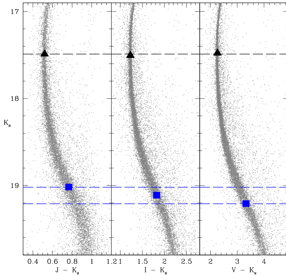
Figure 6.9: Location of the MS-TO (black triangle) and MS-saddle (blue square) in the three CMDs available for NGC 6624. The horizontal black dashed line marks the MS-TO level, the horizontal dashed blue lines the two extreme values of the MS-saddle, which differ by 0.2 mag.
