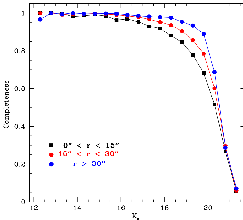
Figure 5.15: Photometric completeness ( \Gamma ) as a function of the K_s magnitude for the GEMINI catalog of NGC 6624 in three different radial bins (see labels).
