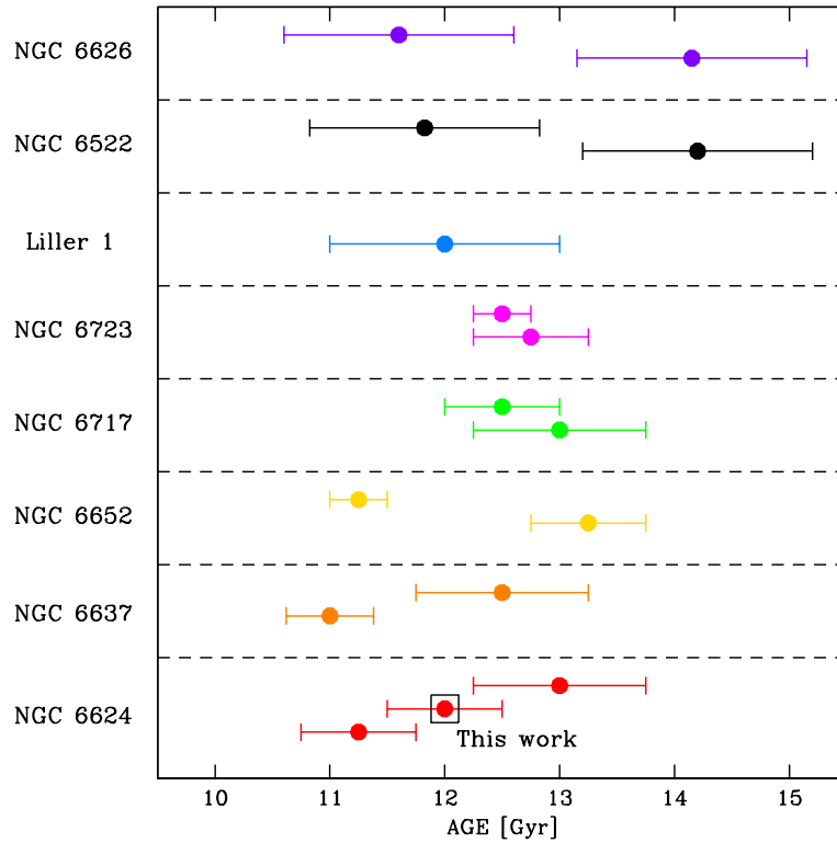
Figure 5.13: The absolute age of NGC 6624 derived in this work is compared to that obtained for other bulge GCs in the literature.
