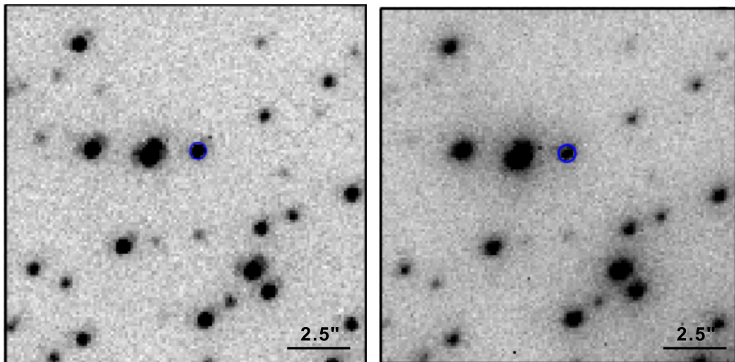
Figure 5.19: Left panel: K_s image of a region of ( 2.5'' \times 2.5'' ) of NGC 6624, centered on the position of StarB, marked with a blue circle, as observed by the GeMS/GSAOI system. This star has the same magnitude as ComStar1 and is adopted for a comparison. Right panel: The same, but in the J band.
