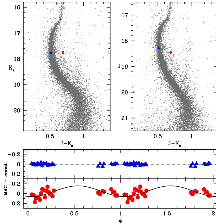
Figure 5.20: Top panels: Positions in the (K_s, J - K_s) and (J, J - K_s) CMDs of ComStar1 and StarB are highlighted with a red circle and a blue triangle, respectively. Bottom panels: The red circles represent the light curve of ComStar1 folded with the estimated orbital period P_{orb} \approx 98 min (Dalessandro et al., 2014). The black line is a sinusoidal function of amplitude \approx 0.2 . For comparison the blue triangles show the light curve of StarB, that has the same average K_s magnitude of ComStar1 but does not show any evidence of flux modulation (dashed black line).
