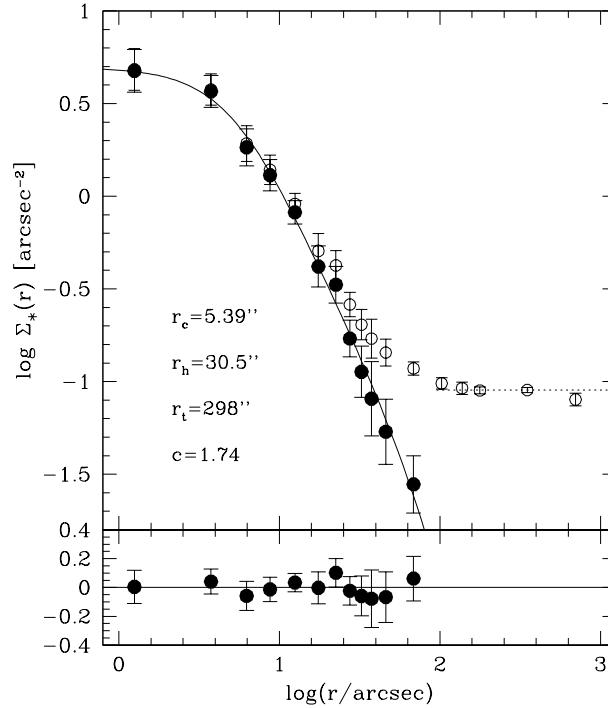
Figure 4.10: Star density profile of Liller 1, obtained from resolved star counts in the combined data set. Empty circles represent the observed profile, while solid ones are obtained after subtraction of the Galactic field density (marked with the dotted line). The best-fit single-mass King model is shown as a solid line and the corresponding structural parameters are labeled in the figure. The lower panel shows the residuals between the observations and the fitted profile at each radial coordinate.
