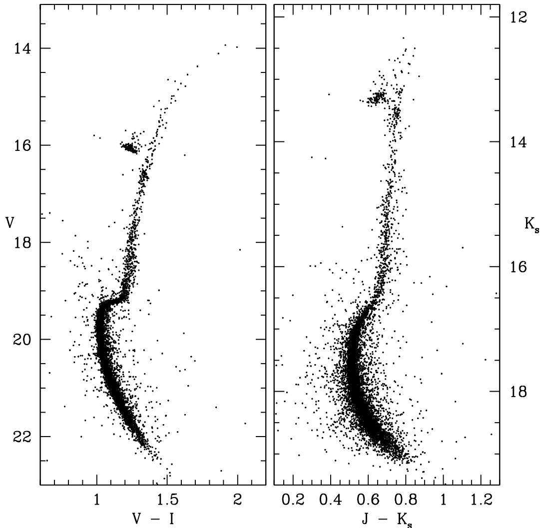
Figure 3.10: V, V - I (left panel) and K_s, J - K_s (right panel) CMDs of the stars in common between the master catalog and the GeMS/GSAOI catalog of NGC 6624 by Saracino et al. (2016).
