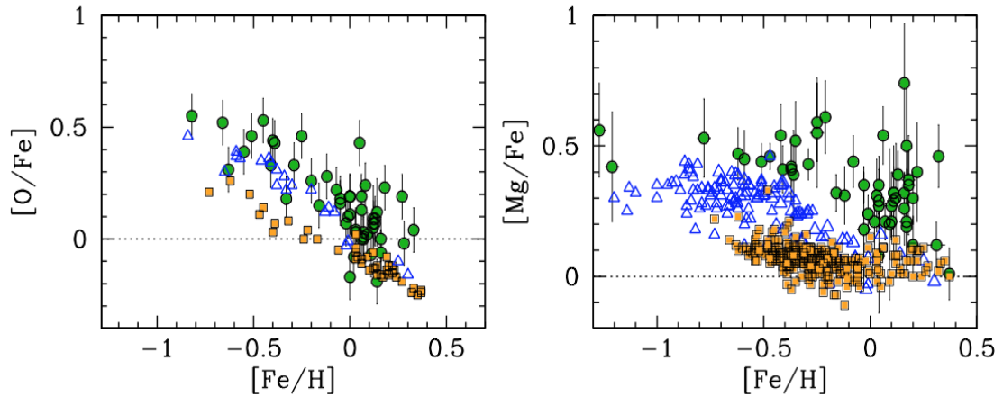
Figure 1.9: Oxygen and magnesium over iron ratios as measured from high dispersion spectra of bulge K giants (Zoccali et al., 2008; Lecureur et al., 2007). Green circles with error bars are bulge stars, compared with thick (blue triangles) and thin (orange squares) disk stars. Figure from Minniti and Zoccali (2008).
