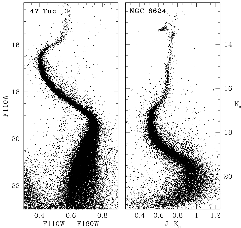
Figure 6.1: Left panel – (F110W, F110W-F160W) CMD of 47 Tucanae from HST observations. Right panel – (K_s, J - K_s) CMD of NGC 6624 from deep observations acquired with a ground-based adaptive optics system.
