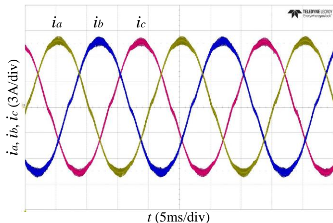
Fig. 22. Three-phase currents with the dead-time of 1.8 \mu s.
