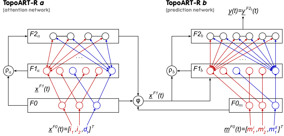
Fig. 2. Structure of TopoART-R. Like TopoART, TopoART-R encompasses two modules (TopoART-R a and TopoART-R b ) sharing the input layer F0 . But the connections of the F2 neurons can either be traced back to \underline{i} or to \underline{d} . Furthermore, TopoART-R b has an additional input control layer ( F0_m ) that is required for prediction.
