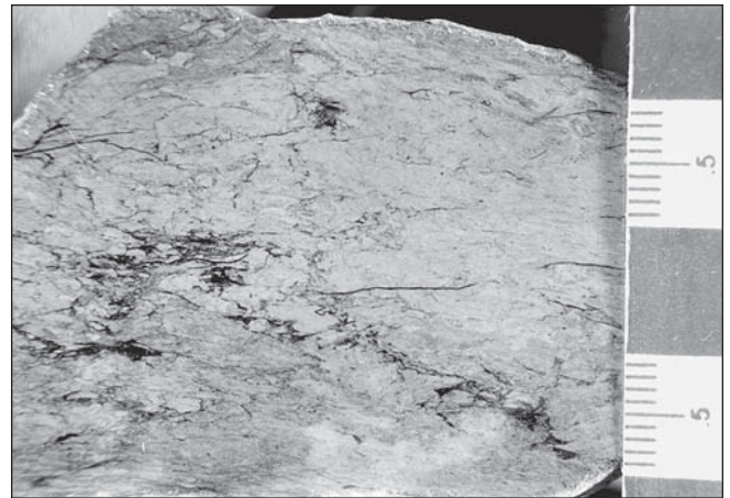
FIGURE 22.—Rock slab of micrite containing abundant coalified macrophytic remains, some within root structures. Stewart section (see fig. 13) on U.S. Rte. 50, Fishpot limestone, Monongahela Group (Virgilian). Scale in centimeters. Photo by K. D. Kallini.
