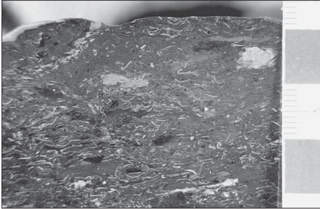
FIGURE 19.—Rock slab of clayey micrite containing ostracode shells. Guysville section on U.S. Rte. 50, Upper Pittsburgh limestone, Conemaugh Group (Virgilian). Scale in centimeters. Photo by K. D. Kallini.
