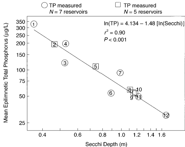
FIG. 1. Relationship between mean total epilimnetic phosphorus concentration (TP) and Secchi depth in Ohio reservoirs, sampled during May through June 1993. Secchi depth was measured weekly in all 12 reservoirs, whereas TP was measured in seven reservoirs (open circles) once every two weeks. Regression analysis on natural-log-transformed data from the seven reservoirs allowed estimation of TP in the five reservoirs in which only Secchi depth was measured (open squares). Reservoirs were ranked from shallowest (1) to deepest (12) Secchi depth (see Table 1).
