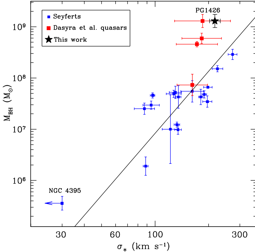
Fig. 3. — The M_{\text{BH}} - \sigma_* relationship for quasars and Seyferts. Blue squares represent Seyfert galaxies, red squares represent quasars studied by Dasyra et al. (2007) using single-slit VLT data, and the star represents the position of PG 1426+015 using the velocity dispersion derived in this work. The black line represents the Tremaine et al. (2002) fit to the quiescent galaxy M_{\text{BH}} - \sigma_* relation.
