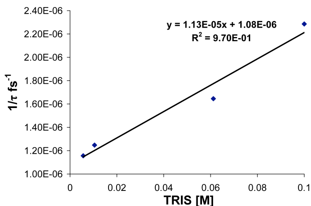
Figure 5. A plot of the observed pseudo-first-order rate constant ( 1/\tau ) of decay of singlet nitrene versus tris-(trimethylsilyl)silane concentration. The nitrene was produced after 260 nm excitation of DPP-N 3 . A single exponential equation was fit to the data obtained from kinetic traces monitored at 550 nm after photolysis.
