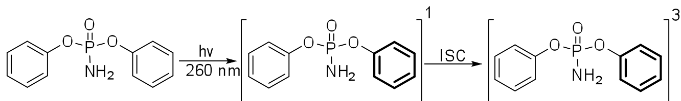
Scheme 3. Ultrafast UV-Vis photochemistry of diphenylphosphoramidate. Note that the lowest energy excited state is localized on the aromatic moiety of this compound.
