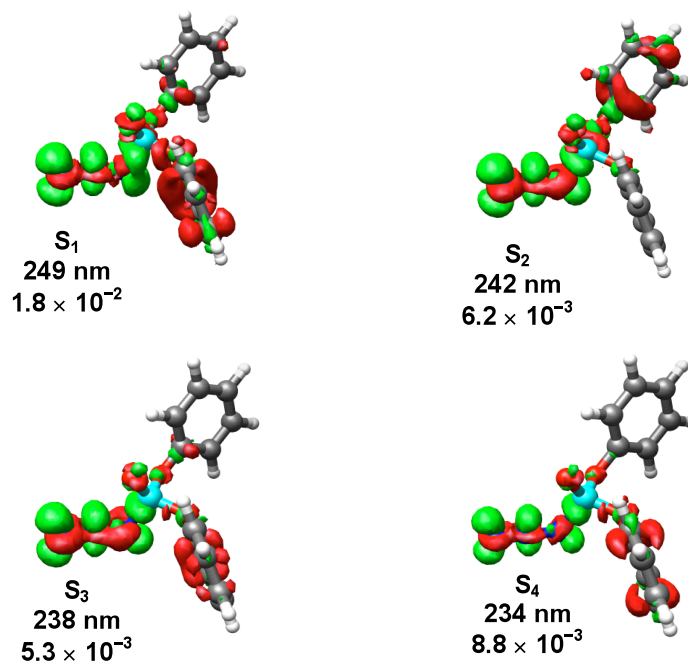
Figure 3. Difference density plots for S_n ( n = 1 to 4 ) of DPP- N_3 at the TD-B3LYP/TZVP level of theory. The energy of the excitation is provided as well as the oscillator strength. The green contours depict the accumulation of electron density in the excited state, and the red contours illustrate the loss of electron density from the S_0 ground state. The isocontour values are \pm 0.003 au.
