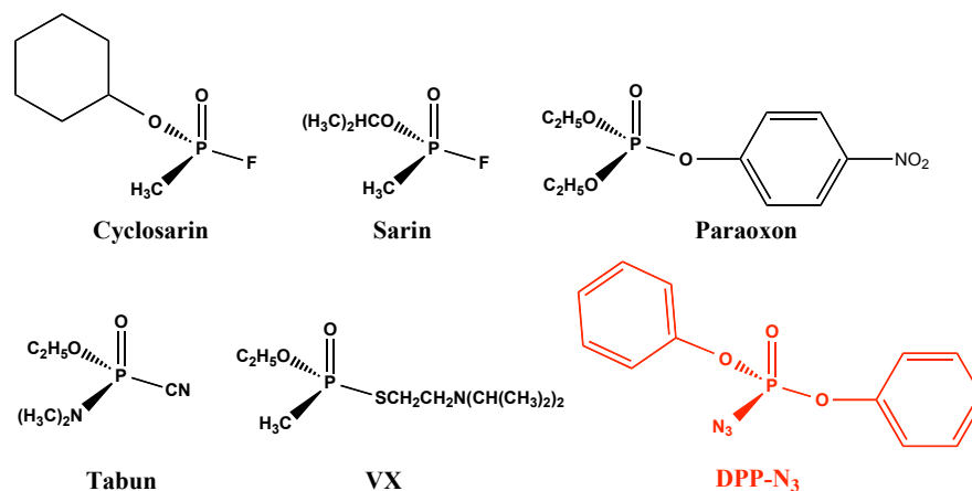
Scheme 1. Some organophosphorus (OP) nerve-agents (in black) and photoaffinity label DPP-N 3 (in red)
