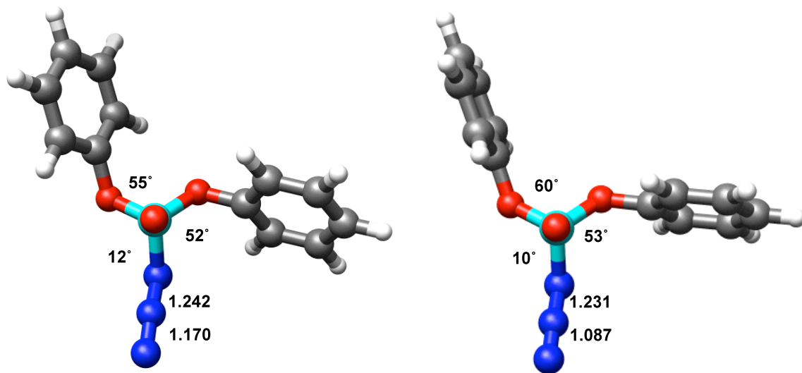
Figure 1. Optimized geometries of diphenylphosphoryl azide (DPP–N 3 ) at the RI-CC2/TZVP (left) and TD-B3LYP/TZVP (right) levels of theory. (Selected distances are shown in Å, and dihedral angles are measured with respect to the O=P bond.)
