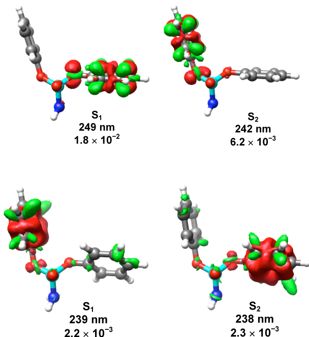
Figure 6. Difference density plots for the S 1 and S 2 states of DPP-NH 2 at the TD-B3LYP/TZVP (top) and RI-CC2/TZVP (bottom) level of theory. The green contours depict the accumulation of electron density in the excited state, and the red contours illustrate the loss of electron density from the S 0 ground state. The isocontour values are -0.005 and +0.0001 au (RI-CC2/TZVP) and \pm 0.001 au (TD-B3LYP/TZVP).
