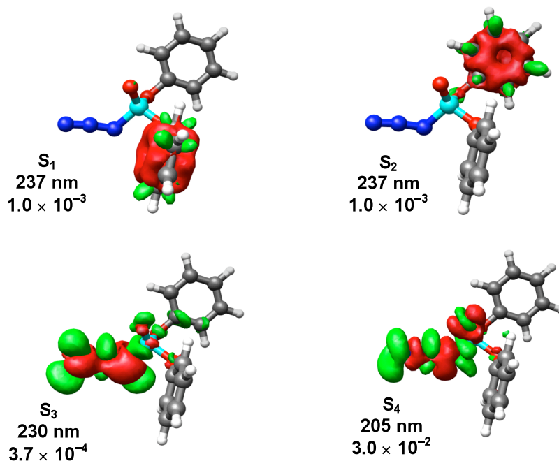
Figure 2. Difference density plots for S_n ( n = 1 to 4 ) of DPP- N_3 at the RI-CC2/TZVP level of theory. The energy of the excitation is provided as well as the oscillator strength. The green contours depict the accumulation of electron density in the excited state, and the red contours illustrate the loss of electron density from the S_0 ground state. The isocontour values are -0.005 and +0.0005 au.
