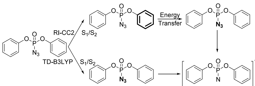
Scheme 2. The photochemistry of DPP-N 3 as predicted by the RI-CC2/TZVP (top) and TD-B3LYP/TZVP (bottom) levels of theory. The initially photoexcited unit of the molecule is depicted in bold.
