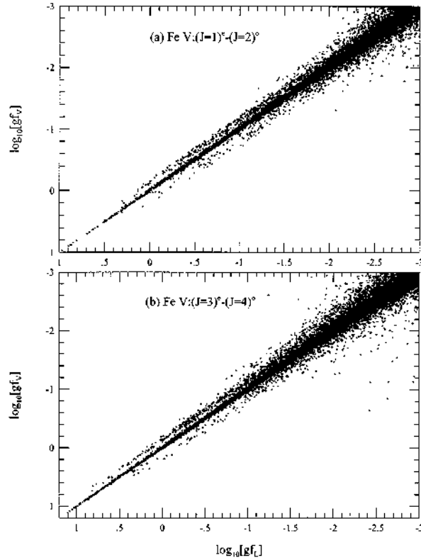
Fig. 1. Comparison of gf_L vs gf_Y for bound-bound fine structure level transitions in FeV obtained in BPRM approximation.
