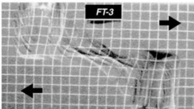
Figure 6: from Dauteuil et al. (2002) showing the different orientations of faults propagation in the experiment. The width of the deformation clearly differing from FT-1 to FT-2 to FT-3.
