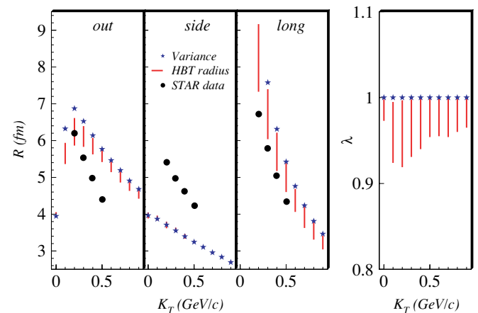
FIG. 16. (Color online) Three-dimensional HBT fit parameters R_{1D,i} and \lambda_{1D,i} as a function of K_T , calculated from the hydrodynamic model using NCE EoS with Eqs. (21). For a given K_T , the vertical red line represents the variation with fit range (see Figure 15). Blue stars represent the corresponding radius parameters calculated from the RMS variances using Eq. (6). Black circles show STAR data [4], with error bars removed for clarity.
