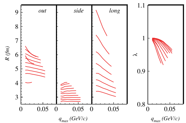
FIG. 15. (Color online) From the hydrodynamic model with NCE EoS, three-dimensional HBT fit parameters R_i and \lambda are calculated with Eqs. (21) and plotted as a function of the maximum allowed value of any q component; see text for details. Each curve corresponds to one of ten values of K_T : 0.0, 0.1, 0.2, ..., 0.9 GeV/c. Curves corresponding to high K_T are at low (high) values of R_i ( \lambda ). The R_l curves for K_T \leq 0.1 GeV/c fall above the plotting range.
