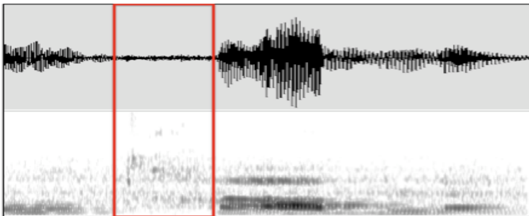
Figure 3: Speaker F1 pronounces a voiceless fricative in the complex onset /tR/ montrable ‘presentable’
