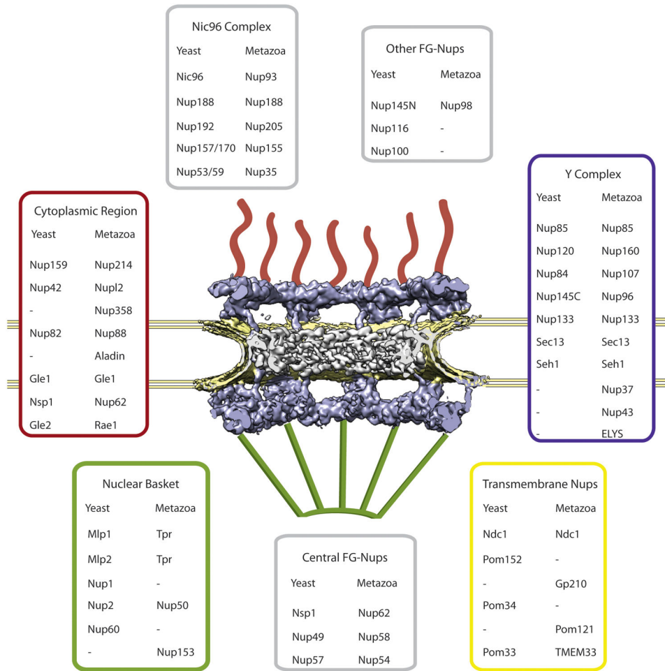
Figure 2. Overall structure of the NPC
