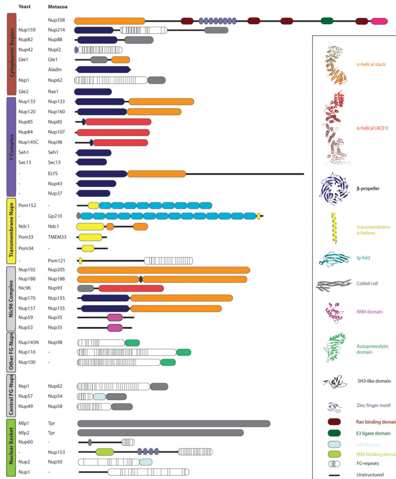
Figure 3. Domain architecture of nucleoporins Yeast nucleoporins with their metazoan homologs are listed. The domain architecture is derived primarily from X-ray crystallographic data, combined with structure prediction whenever experimental data is not yet available. The vast majority of nucleoporins are built from a limited set of structural modules, which characteristically occur in multiple proteins.
