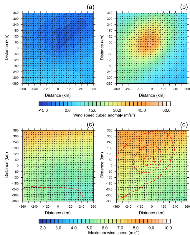
Figure 8. Composites around column rainfall exceeding 1 \text{ mm h}^{-1} . Compositing time includes the point of threshold exceedance and the following 6 h of the simulation. Panels (a, b) show the wind speed cubed anomaly for 12 km simulations with parameterised and explicit convection respectively, arrows represent wind anomaly. Panels (c, d) show composites of the maximum wind speed in the rainfall to rainfall + 6 h window for 12 km simulations with parameterised and explicit convection; arrows represent composite winds and red dashed lines represent wind speed cubed anomaly at 15 \text{ m}^3 \text{ s}^{-3} interval.
