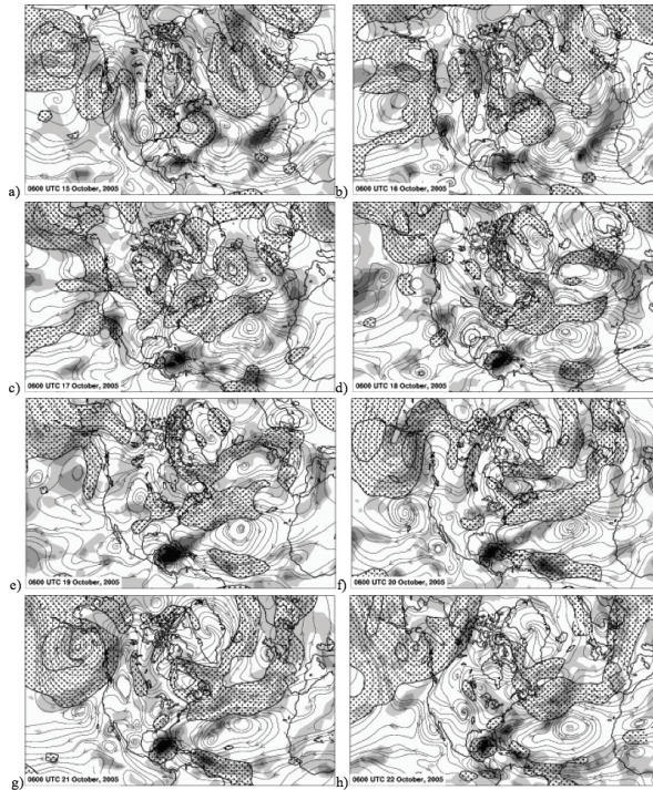
Figure 8. Evolution of the distribution of negative OLR anomalies ( W\ m^{-2} , shaded) during October 15–22, 2005. Stream-line analysis (850 hPa) is superimposed on the low-level wind surge. The contour interval for OLR anomalies is 30\ W\ m^{-2} . Areas of 850 hPa wind surges exceeding 10\ m\ s^{-1} are enclosed by dots within the thick solid contour lines, for which the interval is 15\ m\ s^{-1} .
