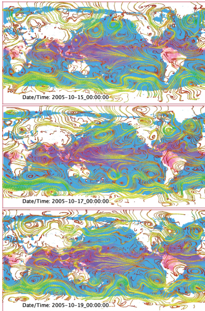
Figure 12. A successful forecast of Wilma's TCG.
