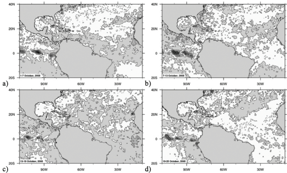
Figure 6. As in Figure 5, except for 6-day changes.
