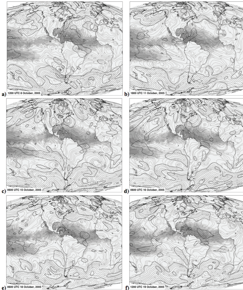
Figure 2. Wind stream analysis (850 hPa) of NCEP/NCAR reanalysis data and NOAA optimum interpolation (OI) 1/4 degree daily sea surface temperature (SST) V2 data superimposed by low-level wind surge at (a) 1200 UTC October 8, (b) 1800 UTC October 11, (c) 0600 UTC October 15, (d) 0600 UTC October 16, (e) 0600 UTC October 18, and (f) 1200 UTC October 19, 2005. Areas of low-level wind surges exceeding 10 \text{ m s}^{-1} are enclosed by dots within the thick solid contour lines, for which the interval is 15 \text{ m s}^{-1} . SSTs exceeding 26^\circ\text{C} are contoured with dark shades at a 1^\circ\text{C} interval.
