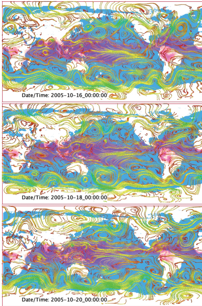
Figure 11. A failed forecast of Wilma's TCG.
