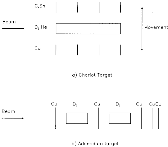
Fig. 2. Schematic diagram of the two target arrangements
