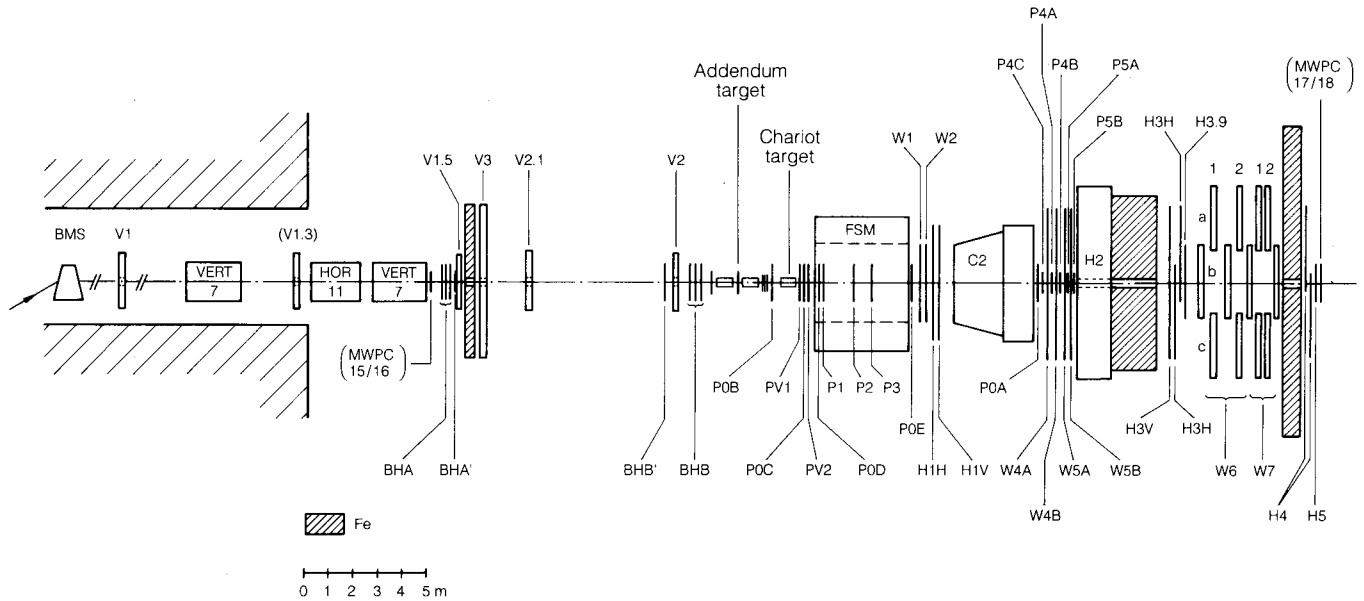
Fig. 1. Schematic diagram of the spectrometer
