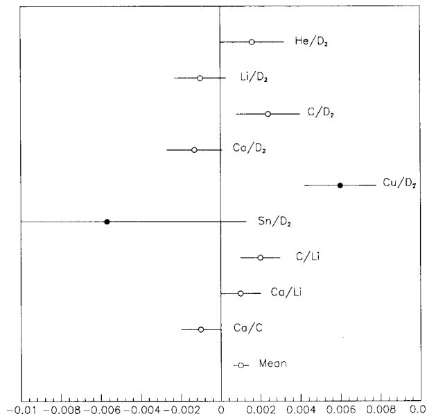
Fig. 9. The total integral over the range x_{\min} < x < 0.30 for all the available data [6, 12, 13 and this experiment]. The lower point shows the mean value, which is compatible with zero as discussed in the text
