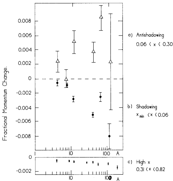
Fig. 8a-c. The integrals \frac{18}{5} \int_{x_{\min}}^{x_{\max}} \left( \frac{F_2^A}{F_2^D} - 1 + f_m \right) F_2^D K_2 dx as a function of A ; a Antishadowing region (triangles) 0.06 < x < 0.30 . The low A data are from [12, 13], the copper data are from this experiment, the Sn data from [6]. b Shadowing region (points) ( x_{\min} < x < 0.06 ) where x_{\min} is the lowest value of x for the available data. c High x region 0.31 < x < 0.82 using the SLAC data [4, 30]
