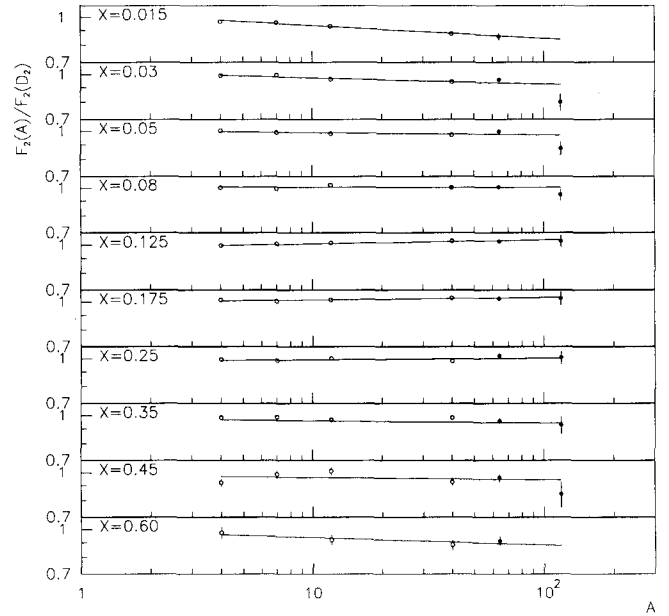
Fig. 6. The structure function ratio as a function of target atomic weight, A . The Cu data are from this experiment (solid circles); the Sn data from [6] and the data at lower A from NMC [12, 13] (open circles). The curves are the results of the fits of the form CA^\alpha
