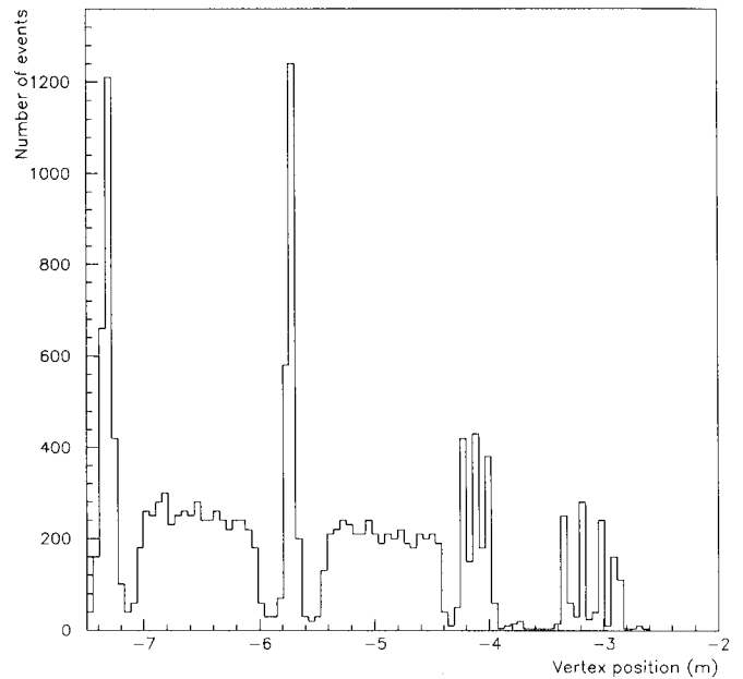
Fig. 3. Reconstructed vertex distribution along the beam direction; the events from each target are clearly identifiable
