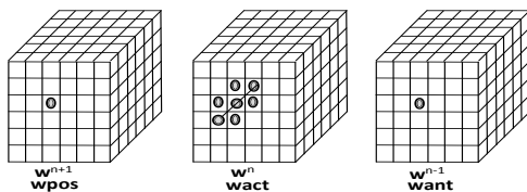
Figure 1: Stencil pattern for 3D-FD of the acoustic diffusion equation model. Based on a multigrid method.
