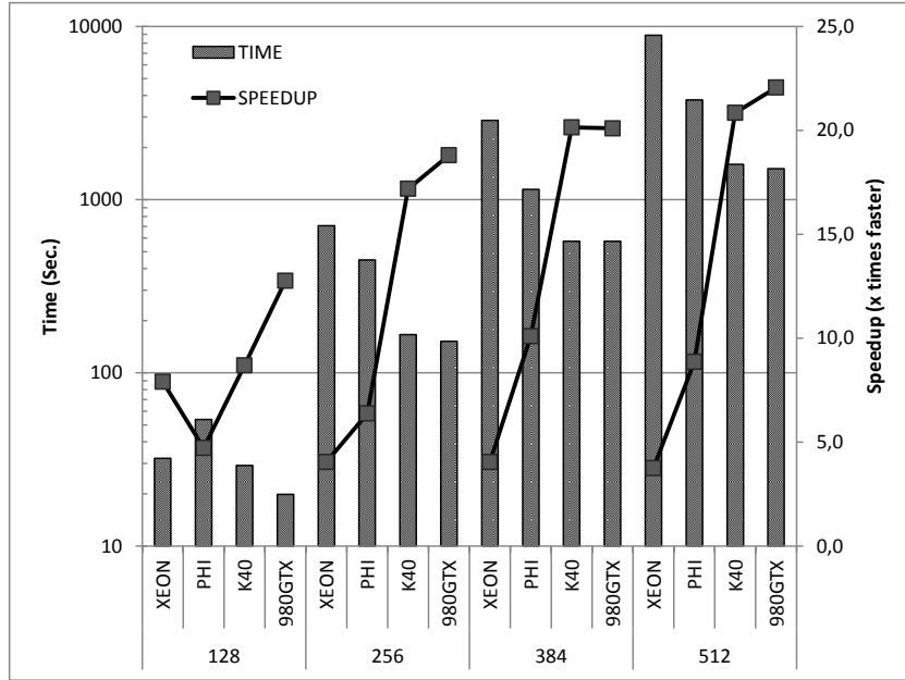
Figure 4: Runtime (prim. Y) and Speedup (sec. Y) for different room resolutions i.e. 128x128x128 (32 MBytes), 256x256x256 (256 MBytes), 384x384x384 (864 MBytes) and 512x512x512 (2048 MBytes) cells.
