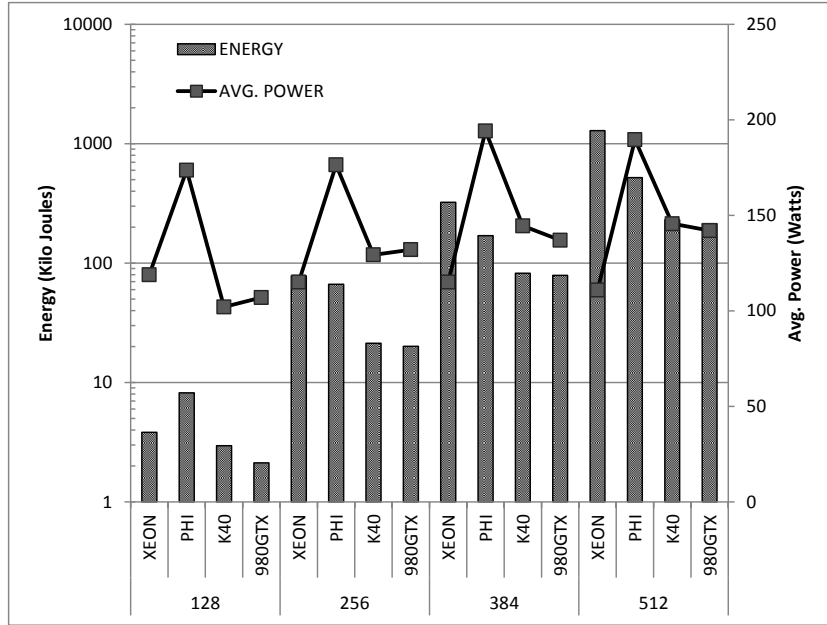
Figure 5: Energy (prim. Y) and Average Power (sec. Y) for different room resolutions i.e. 128x128x128 (32 MBytes), 256x256x256 (256 MBytes), 384x384x384 (864 MBytes) and 512x512x512 (2048 MBytes) cells.
