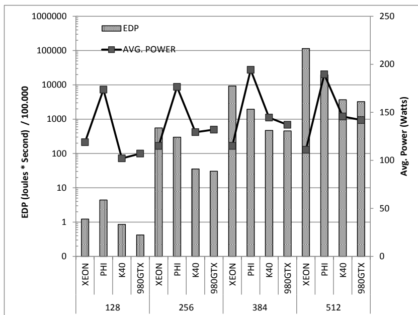
Figure 6: EDP (prim. Y) and Average Power (sec. Y) for different room resolutions i.e. 128x128x128 (32 MBytes), 256x256x256 (256 MBytes), 384x384x384 (864 MBytes) and 512x512x512 (2048 MBytes) cells.
