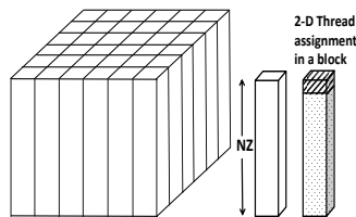
Figure 2: 2D CUDA blocks design. Each CUDA thread need to loop over Z-axis.
