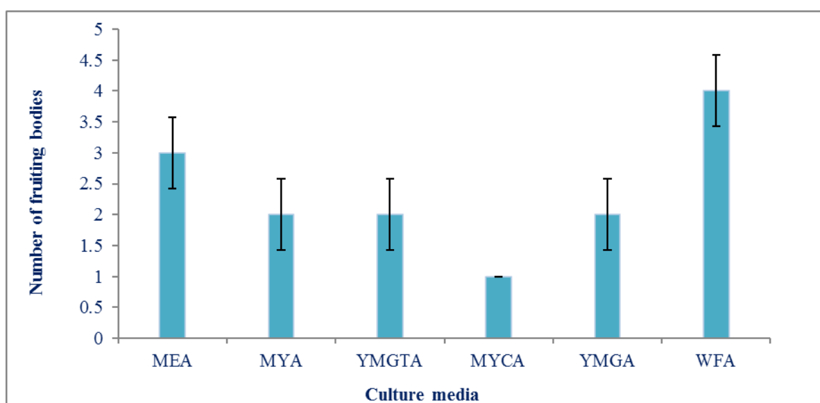
Figs 8 – Fruiting body production of Coprinopsis cinerea strain C2 on different culture media incubated for 15 days at 30° C, pH 6 under dark: MEA- Malt extract agar, MYA- Malt extract yeast extract agar, YMGTA- Yeast extract malt extract glucose tryptophan agar, MYCA- Malt extract yeast extract casamino acid agar, YMGA- Yeast extract malt extract glucose agar and WFA- Wheat flour agar
