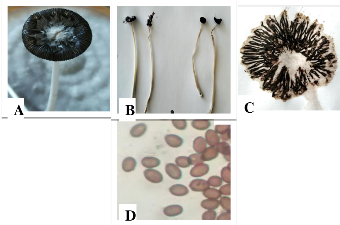
Fig 1 – Fruiting bodies (A, B), spore print (C) and spores (D) of Coprinopsis cinerea
