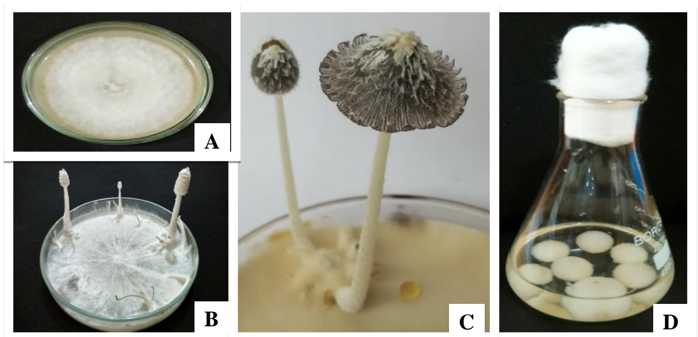
Figs 5 – Growth of Coprinopsis cinerea strain C2 on 2% wheat flour medium incubated for 10 days at 30° C, pH 6 under dark: A) Radial growth B) Fruiting bodies C) Mature fruit body D) Growth on wheat flour broth.
