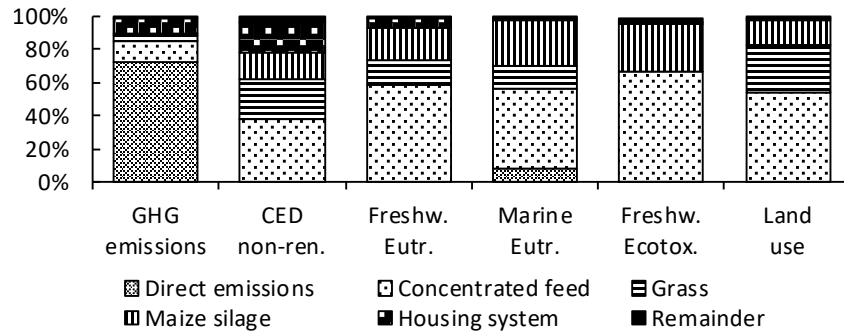
Fig. 2: Contribution analysis of raw milk from Holstein cows at a farm in KwaZulu-Natal analysed in our study (Farm 2) for six impact indicators.
