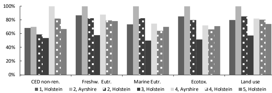
Fig. 4: Comparison of the environmental impact of raw milk at five farms per kilogram milk
