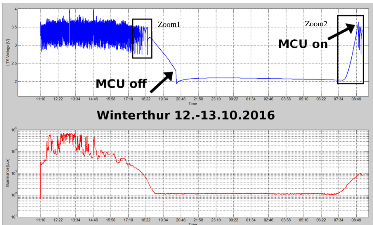
Fig.8 Recording of storage voltage level and transmission activities in function of time of the day. The higher the light intensity, the more transmissions and thus changes of the LTS voltage. Variations on the LTS voltage have to do with the discharge/recharge while transmitting and recharging. This is better seen on the zooms. There are 1013 transmissions in the time interval 11:10 - 18:22 → more than 130 per hour in average Conditions: SF10, RF output power = +14dBm, 868MHz, coding rate 4/5, BW=125KHz Note: The precision of the illumination measurements in the lower end is poor.
