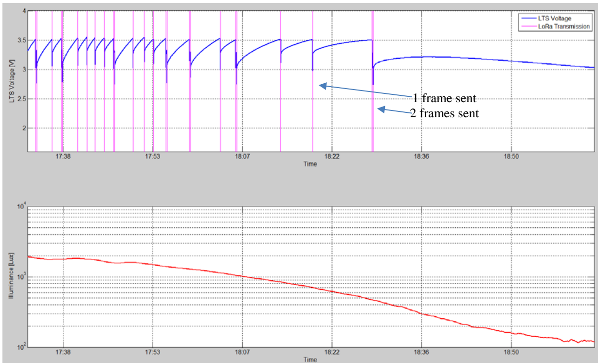
Fig.9 Zoom1 The voltage on the LTS goes down every time a frame is transmitted. Due to a bug, successive frames are sometimes transmitted with 10 seconds interval. Higher illumination means more energy (storage voltage rises faster) and therefore more transmissions.
