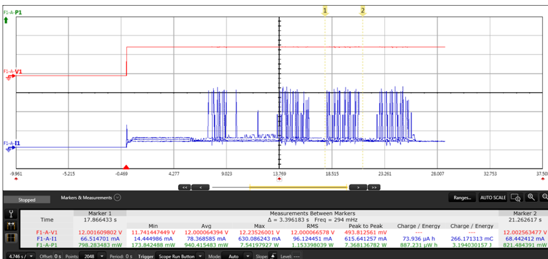
Fig.6 Energy needed to send a message of about 50 character using a GSM modem. More than 3 Joules.
