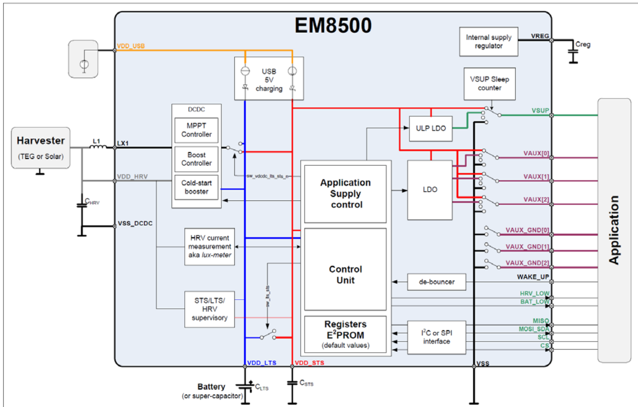
Fig.4 Block diagram of the EM8500. Refer to datasheet for more information [2].
