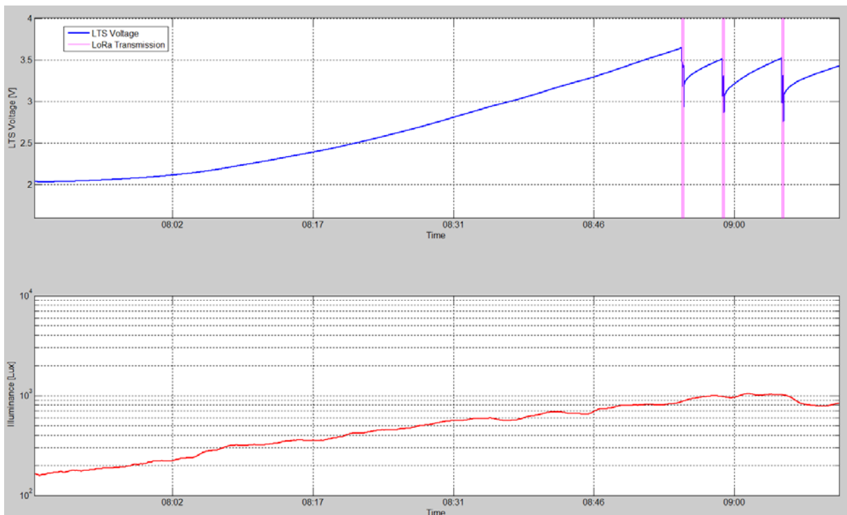
Fig.10 Zoom2 During the night, the storage energy is too low (in this case) to allow any transmission. As the sun rises, energy starts to be accumulated. When there is enough, the embedded system restarts. The system could be dimensioned so that communication is also possible at night, using the stored energy.
