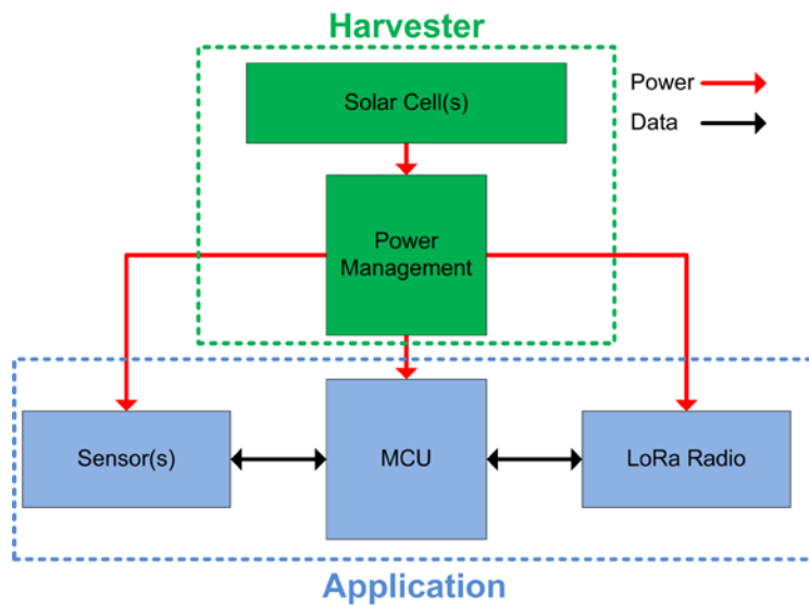
Fig.2 Basic block diagram of the sensing embedded system. The voltage of the solar cell is boosted and the resulting energy is stored in the LTS (Long Term Storage). Converters and other power management elements are used to provide the needed energy to the ES (Microcontroller + LoRa radio) for processing and transmission.
