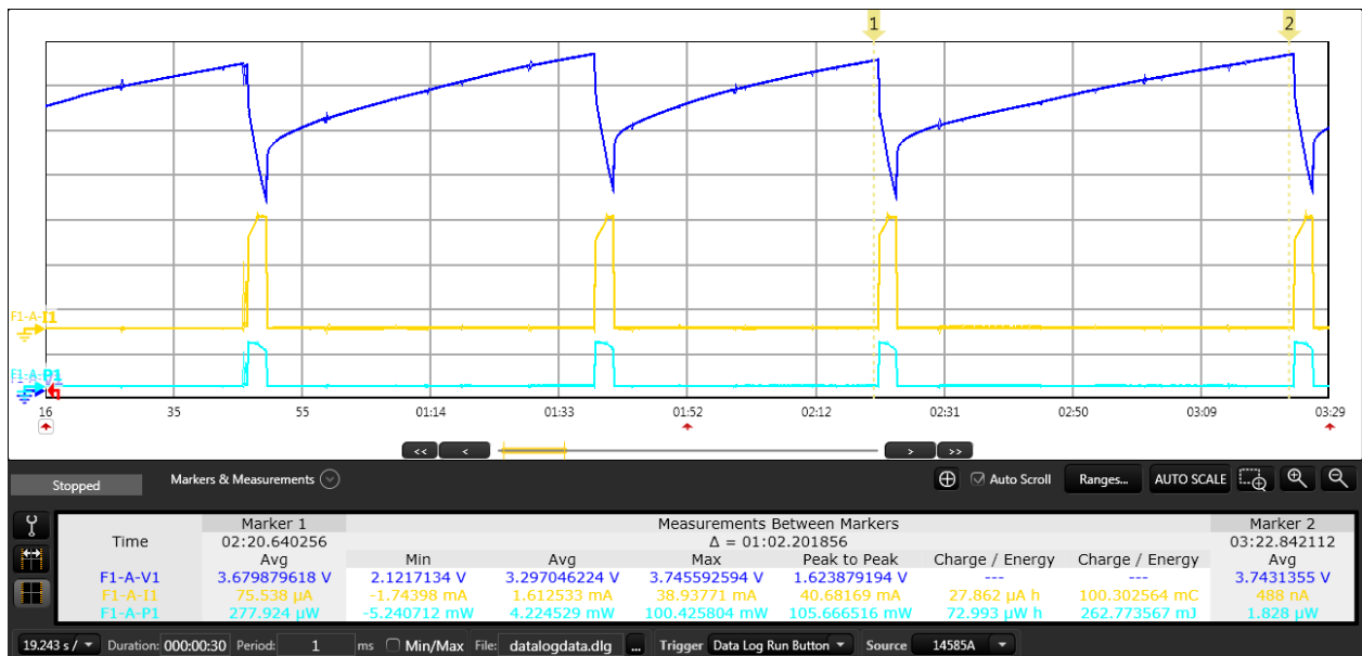
Fig.7 Power profile while transmitting data in SF12 with +14 dBm. 262mJ needed. STS voltage in blue. Current in yellow.
