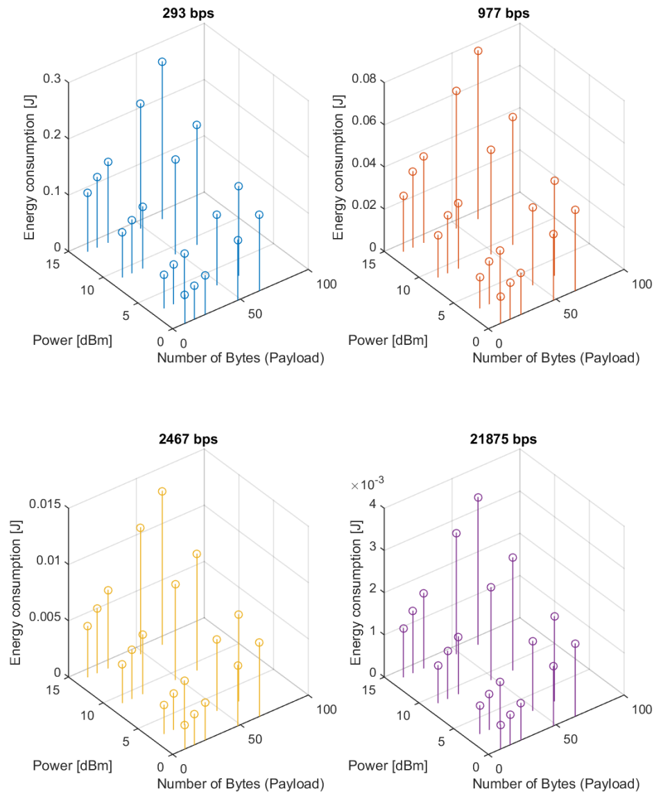
Energy Consumption E(tx\ pwr, n\ Byte, bitrate)
