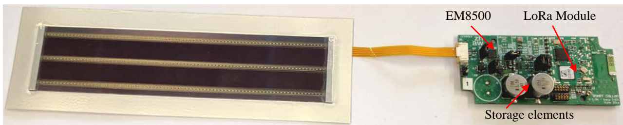
Fig.3. A picture of the embedded system (microcontroller and radio) with an indoor (DSSC) solar cell from GCell. The dimensions of the solar cells are: 167mm x 53mm x 0.5mm (active solar cell area is 140mm x 24 mm) Sensors are from Sensirion, Bosch, Analog Devices. This PCB version with chip antenna
