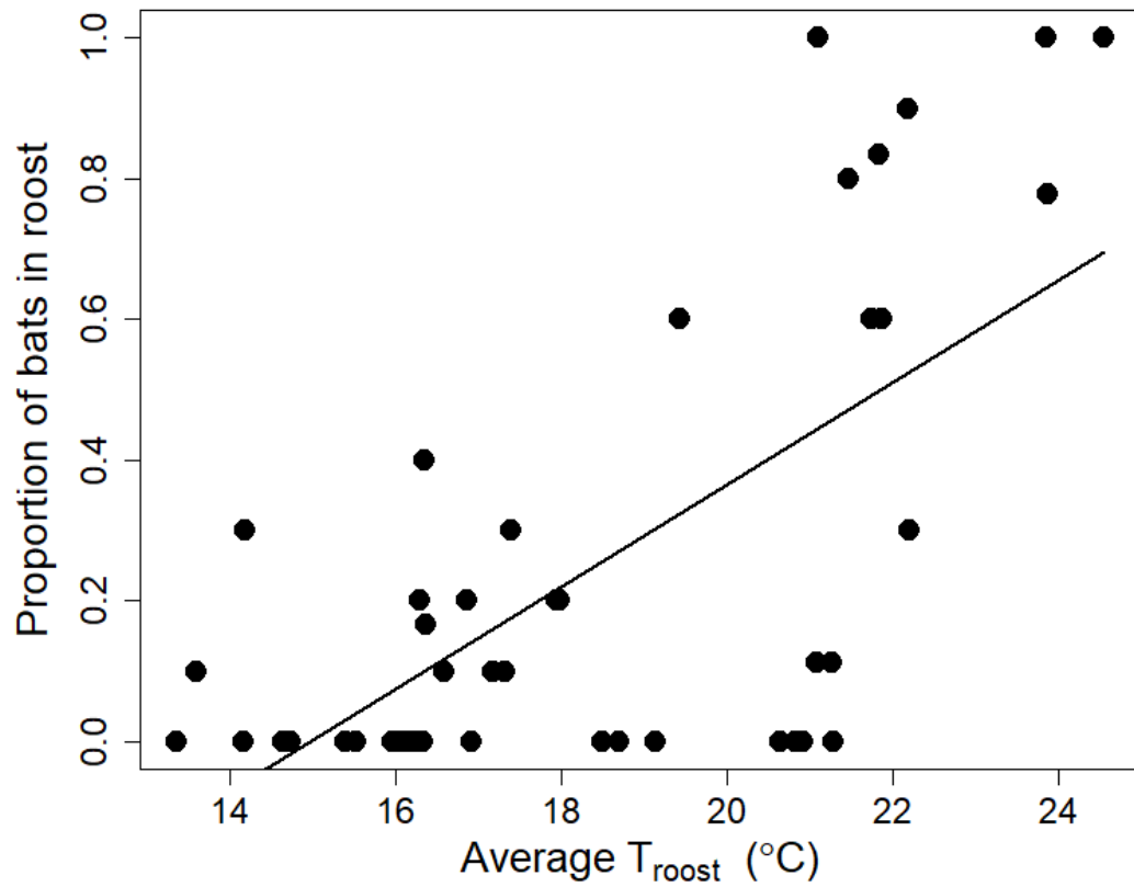
Figure 3.4: Scatter plot of the relationship between the proportion of bats in a roost and daily average T_{\text{roost}} ( ^{\circ}\text{C} ). A linear regression line is also included for illustration although data were analyzed using a generalized linear model (family=binomial, see results).
