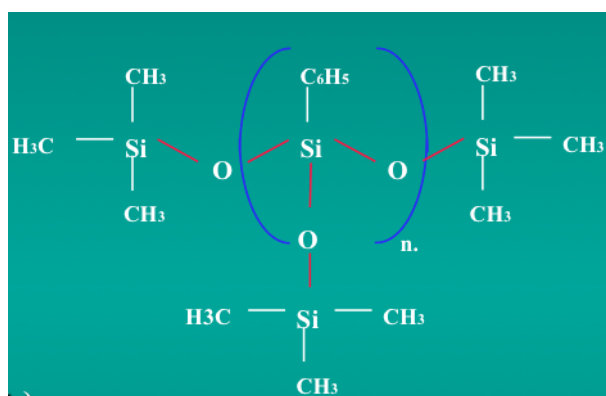
Figure 2.18 : Phenyltrimethicone structure.
