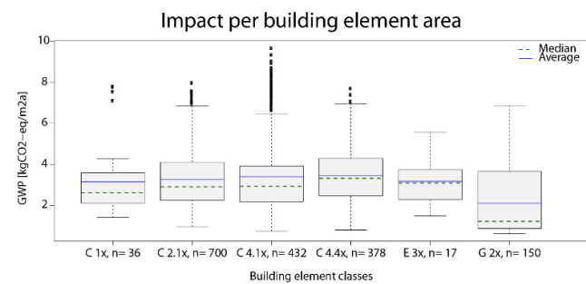
Fig. 5. Comparison of impact per m 2 building element for all construction options
