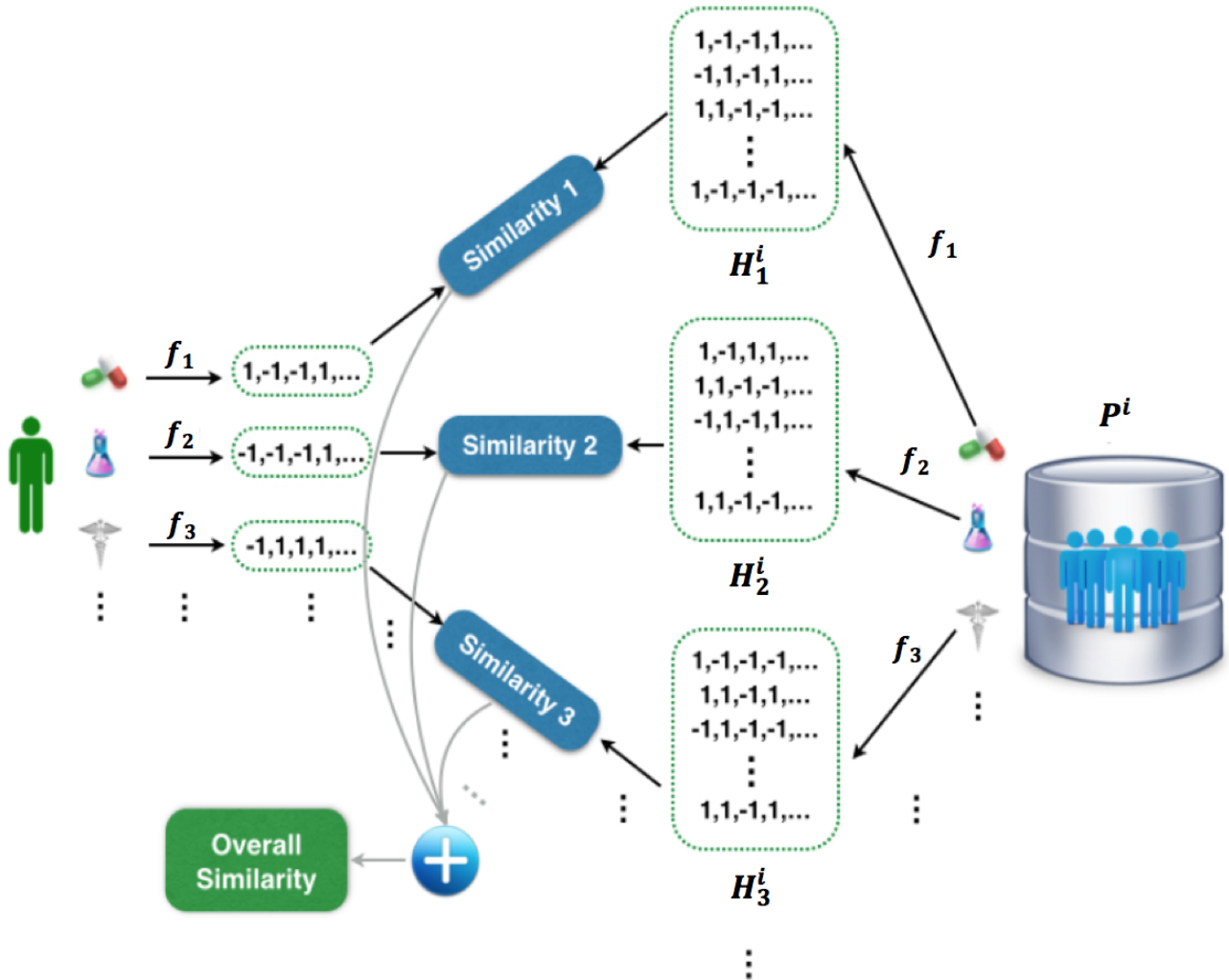
Figure 4. The process of calculating patient similarity with a multi-hash approach.
