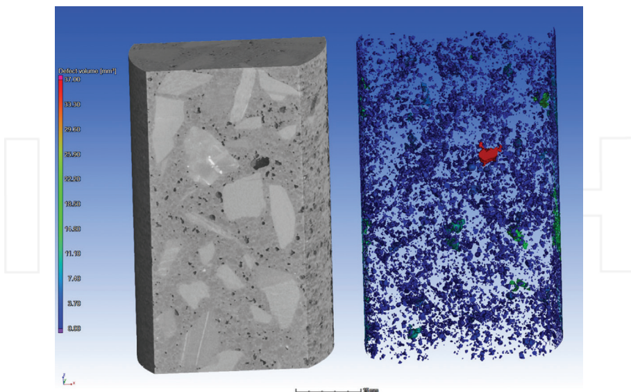
Figure 13. Identification and classification of pores in sizes [61].
