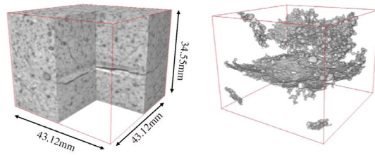
Figure 20. Imaging of fractures that developed at 1000°C [67].
