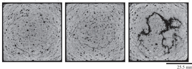
Figure 19. Fracture development at 1000°C [67].
