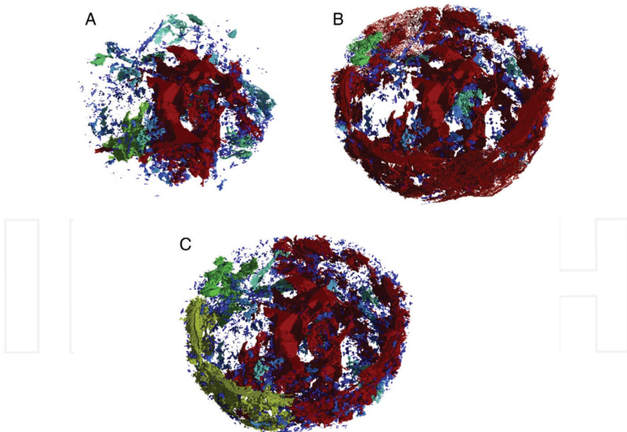
Figure 8. The example of rendering volumes of the changing pores in limestone [35]. The pores are color coded from red (large) to blue (small). Drawing A belongs to unweathered state, drawing B belongs to 6 days of weathering process, and drawing C belongs to 21 days of weathering process.
