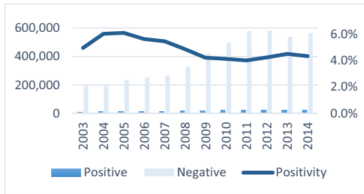
Figure 2 – Longitudinal test results and positivity for chlamydia, gonorrhea and syphilis. Test results are depicted as bars; positivity is depicted as a trend line
