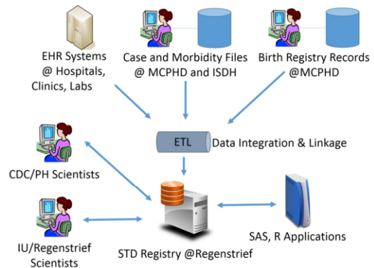
Figure 1 – Diagram depicting data sources, how data are integrated, and how data are accessed for surveillance
