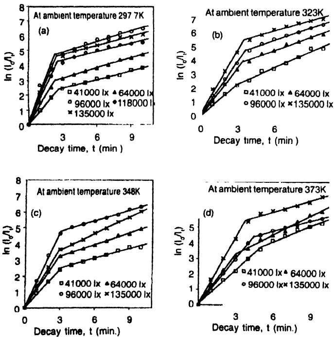
Figure 1. Plots of \ln(I_0/I_t) versus photocurrent decay time ( t ) at different intensity of illumination and ambient temperatures.
