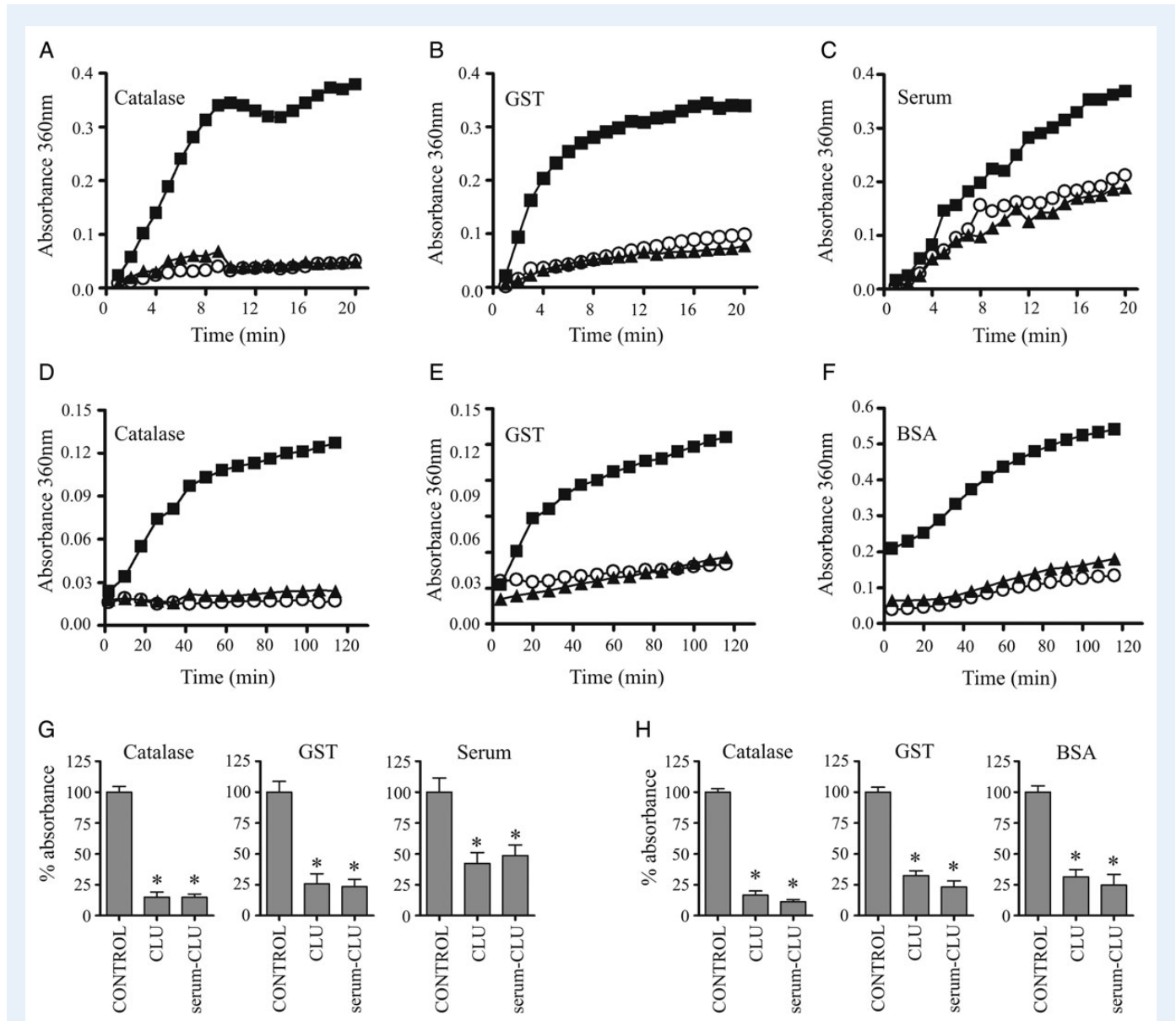
Figure 1 Seminal plasma clusterin has chaperone activity. (A–C) Catalase (200 \mu\text{g}/\text{ml} ), GST (400 \mu\text{g}/\text{ml} ) or human serum (diluted 1 in 10 in phosphate-buffered saline), were incubated for 20 min at 60°C in the presence or absence of seminal plasma clusterin (CLU) (100 \mu\text{g}/\text{ml} ) or serum clusterin (serum-CLU) (100 \mu\text{g}/\text{ml} ). (D–F) Catalase (200 \mu\text{g}/\text{ml} ), GST (400 \mu\text{g}/\text{ml} ) or bovine serum albumin (BSA) (500 \mu\text{g}/\text{ml} ), were incubated for 120 min at 37°C in a buffer containing dithiothreitol (DTT) (20 mM) in the presence or absence of CLU or serum-CLU, at concentrations of 200, 400, or 500 \mu\text{g}/\text{ml} , for catalase, GST, and BSA, respectively. Absorbance at 360 nm was measured at different time points. Squares (■) represent controls, triangles (▲) represent proteins incubated with CLU and circles (○) represent proteins incubated with serum-CLU. Representative experiments are shown ( n = 3–6 ). (G and H) Experiments in (G) and (H) were performed as described above for (A)–(C) (20 min at 60°C), and (D)–(F) (120 min at 37°C with DTT 20 mM), respectively. Results are expressed as the mean \pm SEM of 3–6 experiments. The absorbance of stressed-proteins incubated with CLU or serum-CLU was expressed as the percentage of the absorbance of proteins stressed in the absence of clusterin (CONTROL). * P < 0.01 versus CONTROL (student's t -test).
