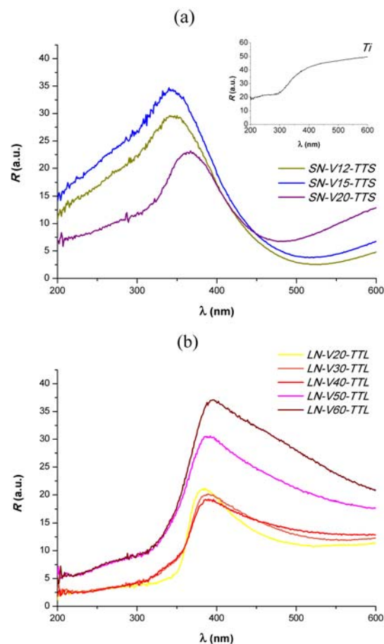
Fig. 3. UV-Vis diffuse reflectance spectra of selected samples: (a) SN and (b) LN.
