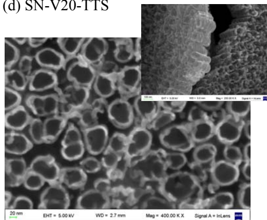
Fig. 1. SEM micrographs of the top of the SN coatings obtained at different voltages. Inset in Fig. 1(d): cross-sectional view of the corresponding coating.
