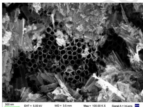
(c) LN-V40-TTL
