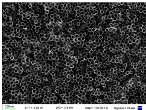
(a) LN-V20-TTL
