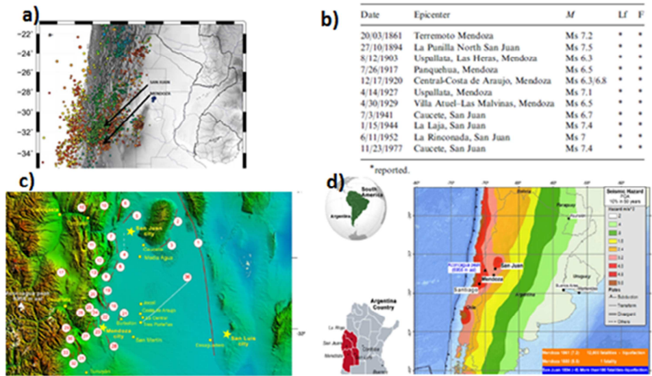
Fig 1: (a)-seismicity map of Cuyo region (INPRES) and (b)-catastrophic historical events with liquefaction (Lf) and cracks (l) (Moreiras 2004) (c) active faults at the piedmont of the central Argentinian Andes (Moreira 2014). (d) Potential ground motion for Argentinean local and subduction Chilean earthquakes in Moreiras (2014 from USGS)
