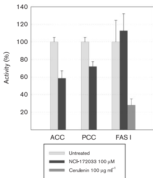
Fig. 6. In vivo effect of NCI-172033 on the ACCase, PCCase and FAS I activities of M. smegmatis . Cultures of M. smegmatis were incubated in the presence of 100 μM NCI-172033 and the relative acetyl- and propionyl-CoA-dependent carboxylases and FAS I activities determined in the cell-free extracts. Cerulenin, a known inhibitor of the β-ketoacyl synthase domain in type I synthases, was used as a control.
