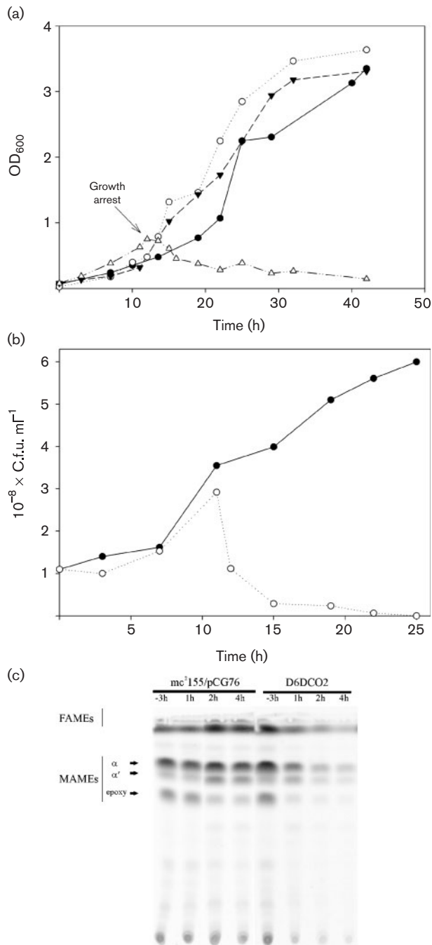
Fig. 2. Growth characteristics and lipid composition of the accD6 conditional mutant D6DCO2 incubated at 30 and 42 °C. (a) Growth curves of strains mc 2155 / pCG76 (●, ○) and D6DCO2 (▼, △) incubated at 30 °C (black symbols) and 42 °C (white symbols). Saturated cultures grown at 30 °C were diluted in fresh 7H9 medium supplemented with ADS to an OD 600 of 0.1 and further incubated at 30 or 42 °C. The arrow indicates growth arrest of D6DCO2. (b) At different time points, the number of viable cells of D6DCO2 in the cultures grown at 30 °C (●) and 42 °C (○) was evaluated by plating serial dilutions onto LB plates at 30 °C. (c) Saturated cultures of strains mc 2155 / pCG76 and D6DCO2 were diluted in fresh 7H9 medium and incubated at 42 °C. At -3, 1, 2 and 4 h before or after D6DCO2 stopped growing (see a), aliquots from both cultures containing the same number of cells were labelled with [ 14 C]acetate for 1 h at 42 °C. One half of each sample was used to study the fatty acid and mycolic acid compositions of the strains by TLC (solvent system: hexane/ethyl acetate, 10:1).
