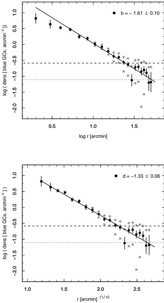
Fig. 6. Radial density profiles for blue GC candidates in the field of NGC 1399 showing power law (upper panel) and r^{1/4} fits (lower panel) to the data. Filled circles show the background-corrected distribution of blue GC candidates, while plus signs and crosses show the same distribution considering a background 50 per cent higher and 50 per cent lower, respectively, than the original one. The dashed lines correspond to the background projected density and the dotted lines to 30 per cent of the background density. The coefficients in the upper right corners give the slope of the corresponding fits.
