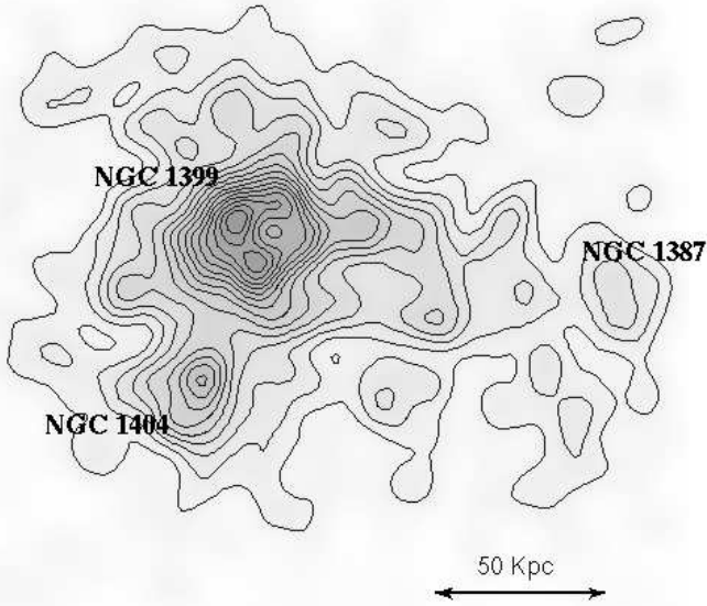
Fig. 9. Smoothed, projected distribution of blue GC candidates around NGC 1399. Solid lines correspond to curves with constant numerical density. North is up and East to the left.
