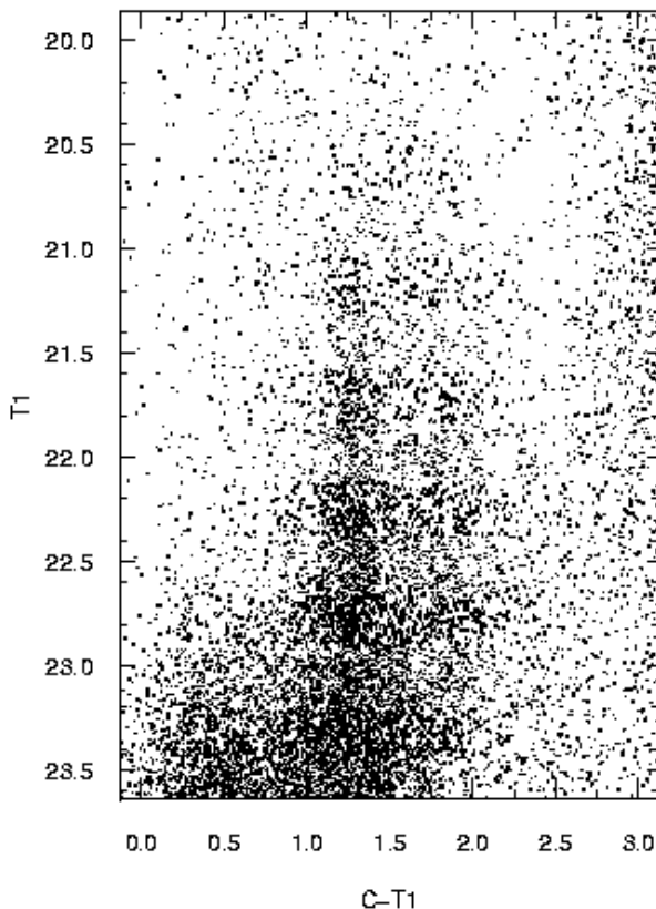
Fig. 2. Colour-magnitude diagram for all point sources in the MOSAIC field. Globular cluster candidates show up in the colour range 0.8 \leq (C - T_1) \leq 2.3 . The dense group of objects bluer than (C - T_1) = 0.8 and fainter than T_1 = 23 are mainly compact background galaxies.
