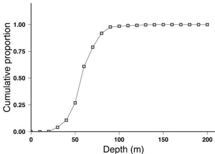
Figure 6. Upper panel , relative density (survey CPUE) of immature female snow crab integrated over time from 1978 to 2001. Lower panel , cumulative proportion of immature females (number sampled weighted by abundance) relative to depth (NMFS survey data).
