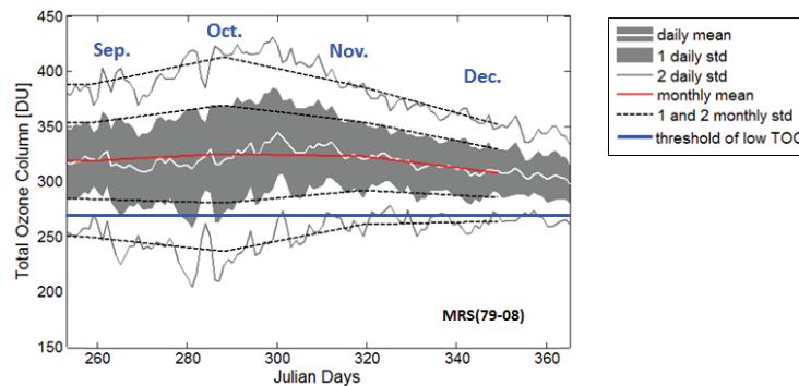
FIGURE 2. Total Ozone Column Climatology (1979 – 2008) [8]
