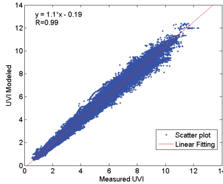
FIGURE 1. Scatter plot and linear fitting between UVI_{mod} and UVI_{GUV} .
