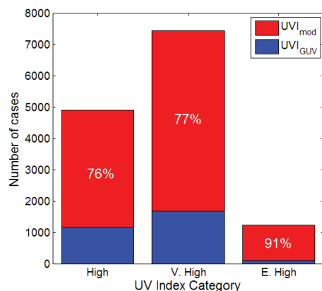
FIGURE 3. Number of cases (minutes) that reach each category for UVI mod (red) and UVI GUV (blue)
