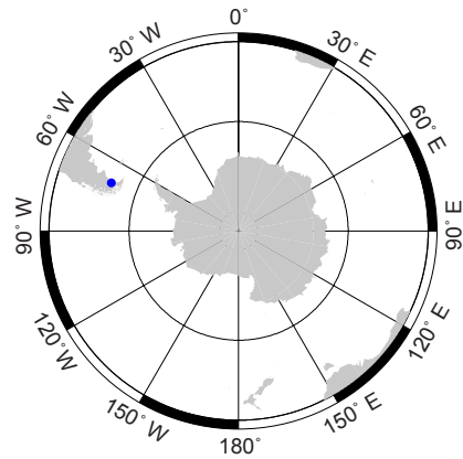
Figure 1. Location of the OAPA site in Río Gallegos, Argentina, (51.6° S, 69.3° W), shown as a blue circle. Latitude ranges from 30 to 90° S.
