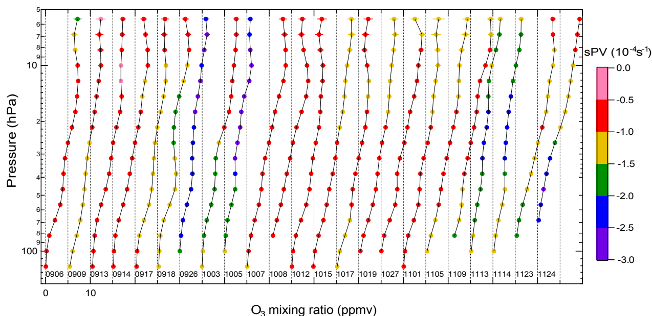
Figure 3. Time series of DIAL O_3 profiles at the OAPA site. Each profile is shifted 5 ppmv. Data are color coded based on sPV values. Observation dates in 2009 are shown as MMDD (e.g., 0906 is 6 September 2009).
