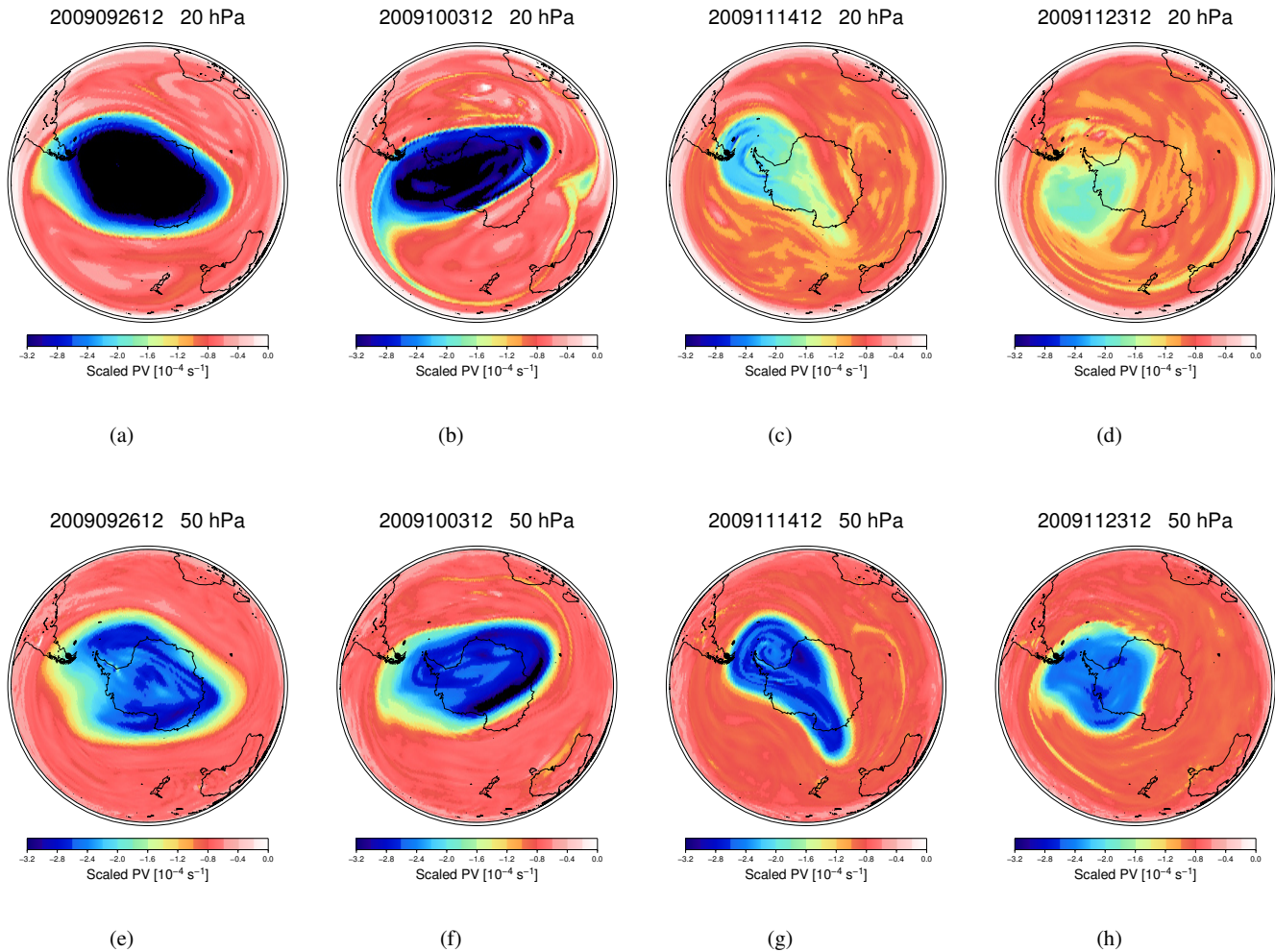
Figure 4. Scaled PV maps from MERRA-2 on 26 September (a, e), 3 October (b, f), 14 November (c, g), and 23 November 2009 (d, h). Top and bottom rows show pressure surfaces at 20 and 50 hPa, respectively.
