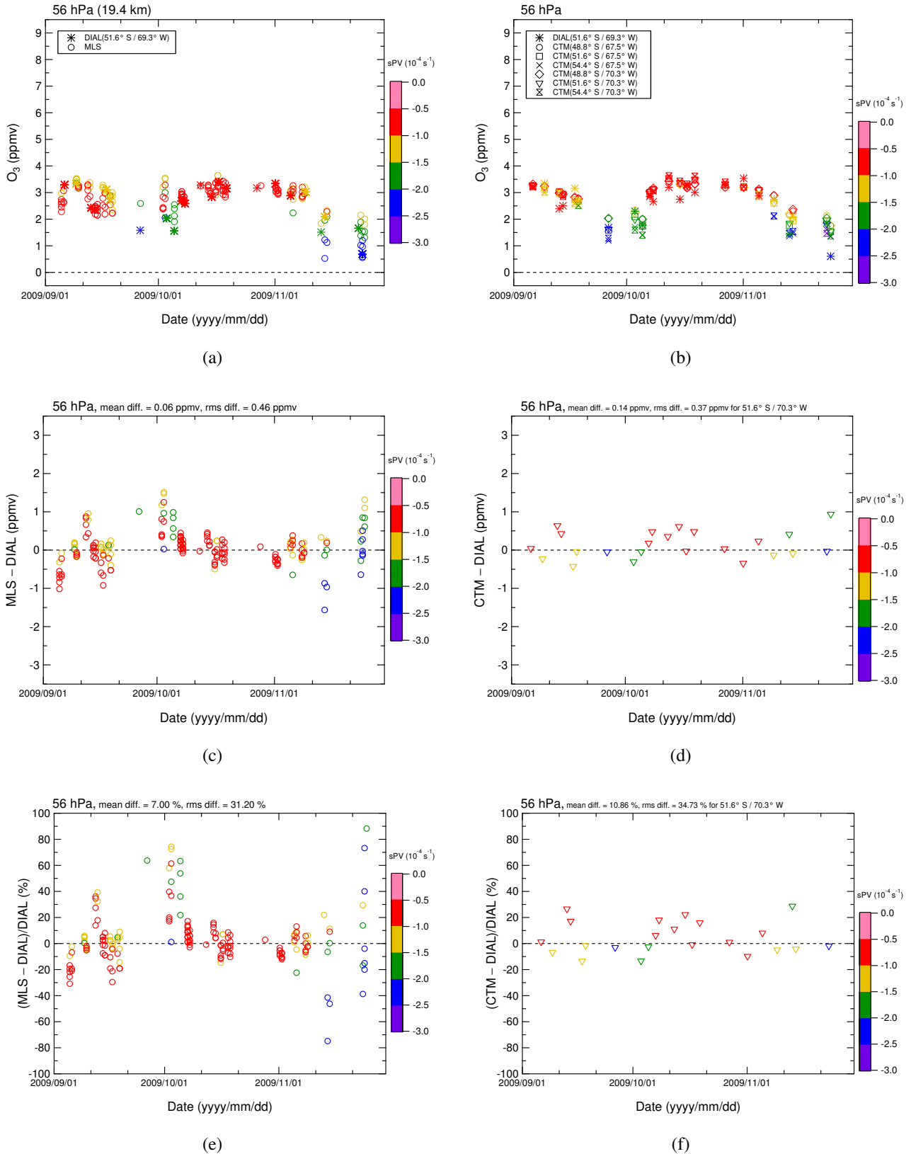
Figure 6. Time series of O 3 mixing ratios as measured by DIAL and MLS at 56 hPa (a) and absolute and relative differences between the two (c, e) from September to November 2009, over the OAPA site. Panels (b) and (d, f) are the same as panels (a) and (c, e), but for DIAL and MIROC-CTM. Data are color coded based on sPV values. For the absolute and relative differences, sPV values for MLS and MIROC-CTM are color coded. For MIROC-CTM, outputs from six grids are shown (see text for additional description).
