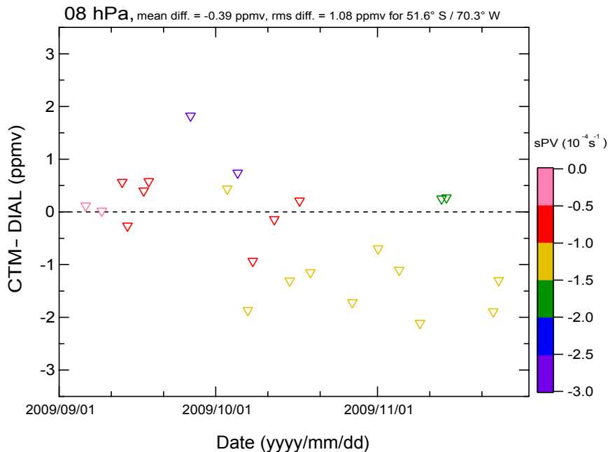
Figure 12. Time series of differences in O_3 mixing ratios as measured by DIAL and computed by MIROC-CTM at 8 hPa from September to November 2009, over the OAPA site. Data are color coded based on sPV values for MIROC-CTM.
