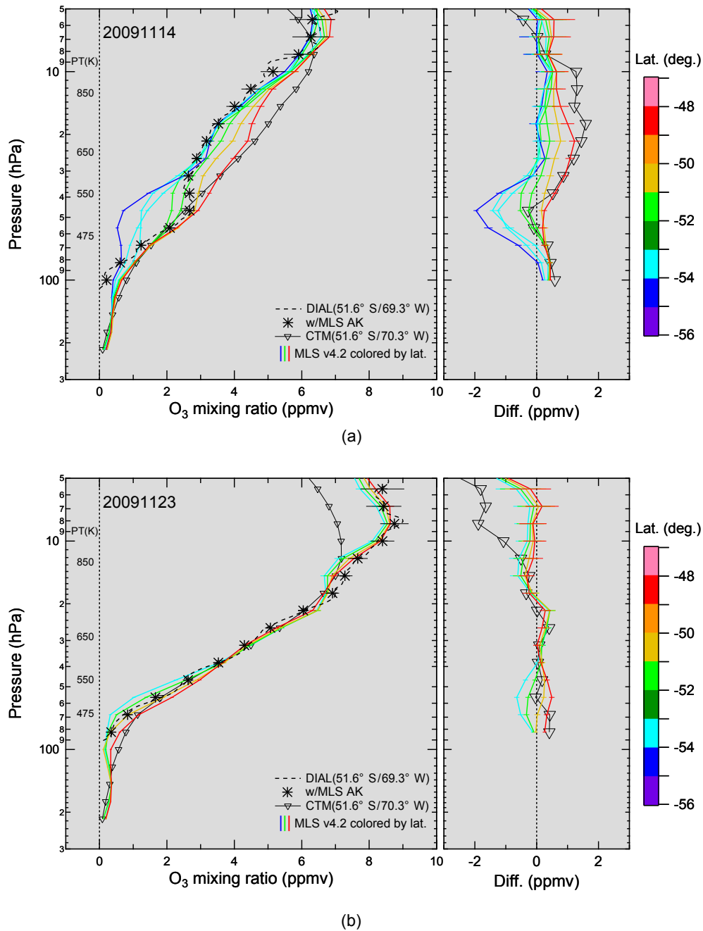
Figure 2. Vertical profiles of O 3 mixing ratios on 14 November 2009 (a) and 23 November 2009 (b) measured using DIAL (asterisks and dotted line) and MLS (solid lines with color) over the OAPA site (see text for additional description). A MIROC-CTM O 3 profile of the nearest grid for the OAPA site is also shown. Corresponding potential temperatures for pressure are shown as text in the vertical axis. Differences between DIAL and X (MLS or MIROC-CTM) ( X - \text{DIAL} ) are shown in the right panel (see text). The MLS profiles are color coded based on their measurement latitudes.
