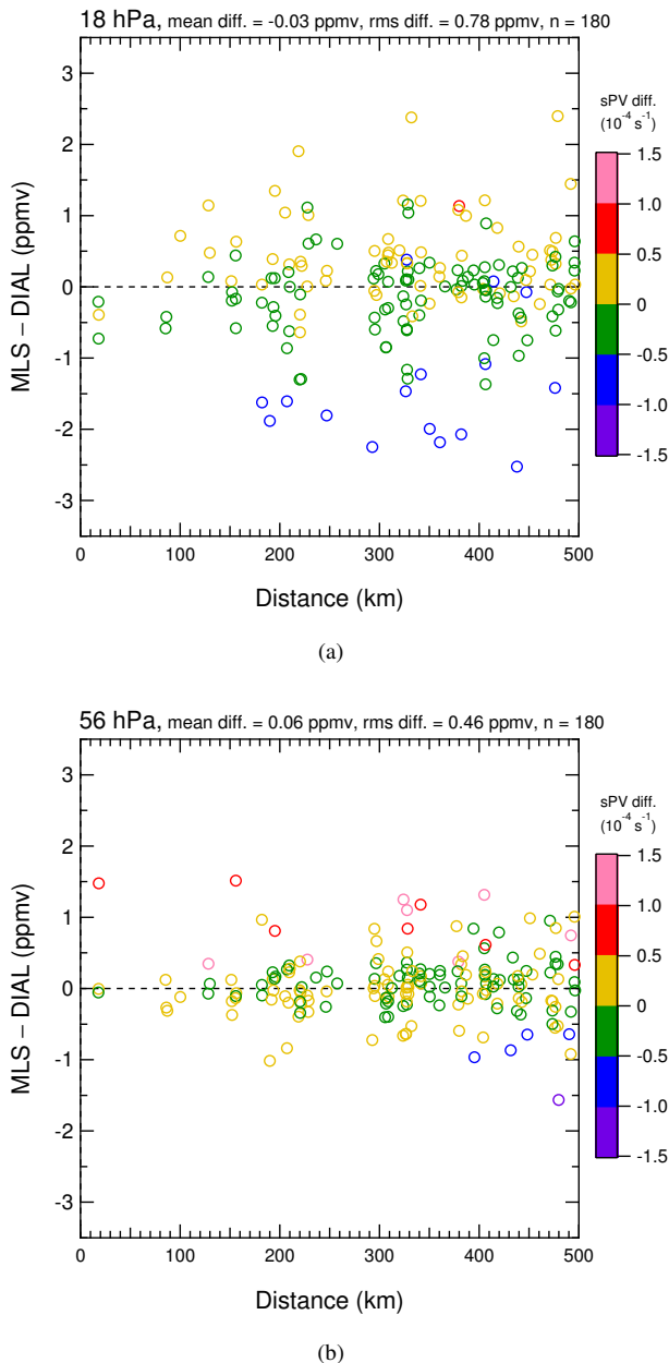
Figure 9. O 3 difference versus distance for DIAL and MLS at 18 hPa (a) and 56 hPa (b). Data are color coded based on sPV differences between DIAL and MLS measurements.
