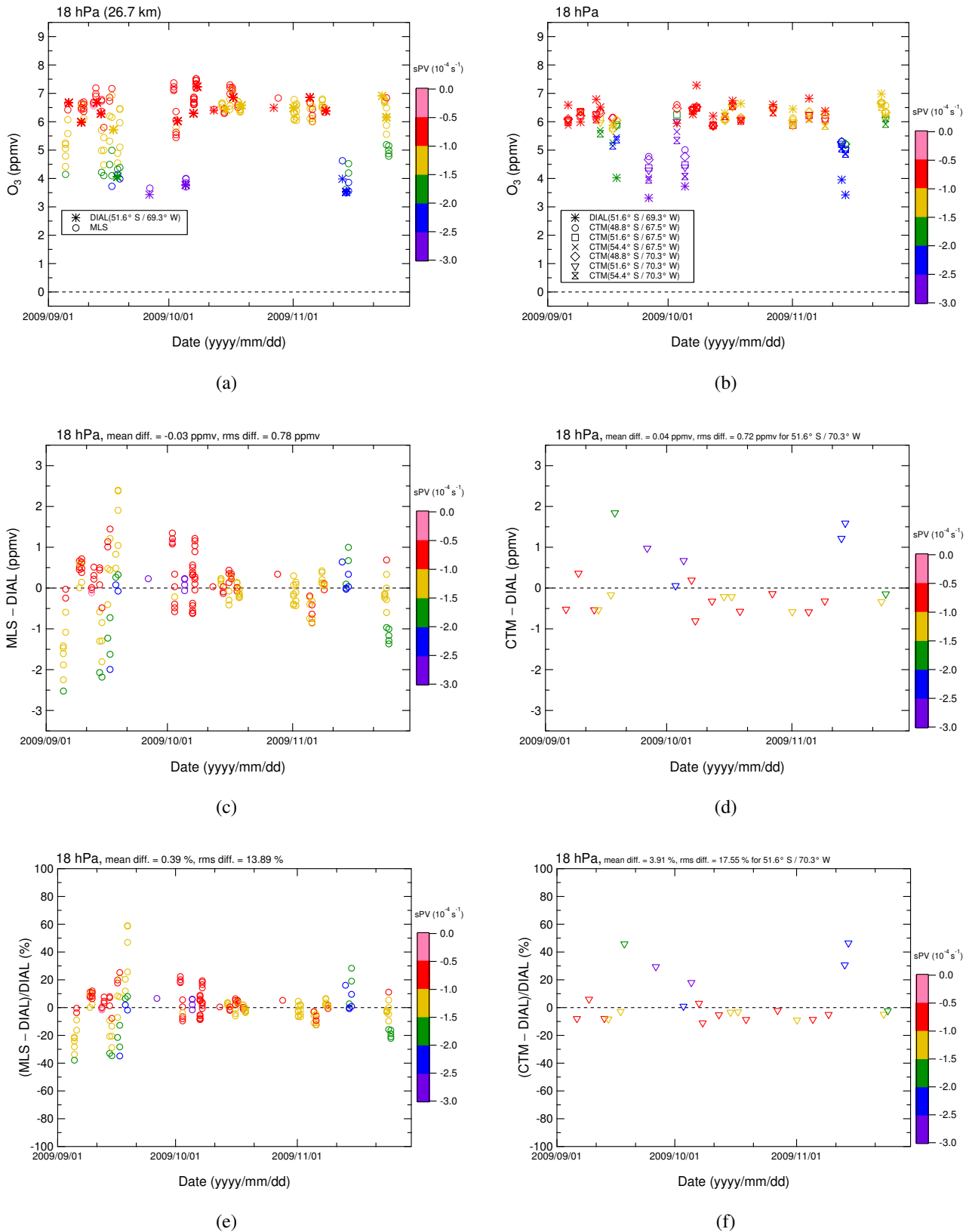
Figure 5. Time series of O 3 mixing ratios as measured by DIAL and MLS at 18 hPa (a) and absolute and relative differences between the two (c, e) from September to November 2009, over the OAPA site. Panels (b) and (d, f) are the same as panels (a) and (c, e), but for DIAL and MIROC-CTM. Data are color coded based on sPV values. For the absolute and relative differences, sPV values for MLS and MIROC-CTM are color coded. For MIROC-CTM, outputs from six grids are shown (see text for additional description).
