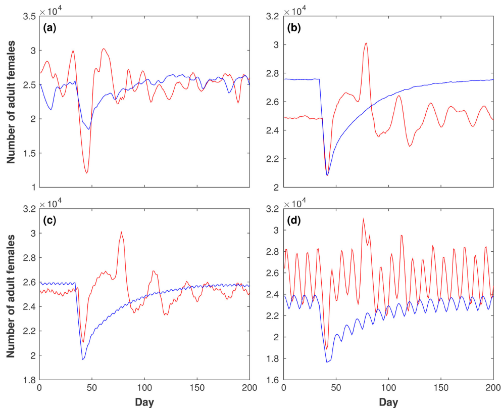
Fig. 3. Effect of a 1-week drop in temperature on the number of adult females. A sudden drop in temperature from 25.8^{\circ}\text{C} (the annual average) to 20^{\circ}\text{C} is simulated between days 35 and 41 inclusive, under various rainfall regimes: (a) actual daily rainfall, (b) rainfall every day, (c) rainfall every 4 d, and (d) rainfall every 10 d. The amount of daily rainfall is adjusted in the periodic regimes so that the annual total is the same across all four regimes. Plotted curves correspond to the time course of the number of adult females according to the Skeeter Buster model (red curves) and the AedesBA model (blue curves). All results shown are averages over 20 simulation runs.
