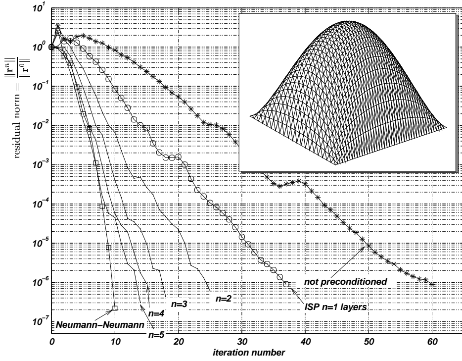
Fig. 8. Solution of Poisson's problem.
