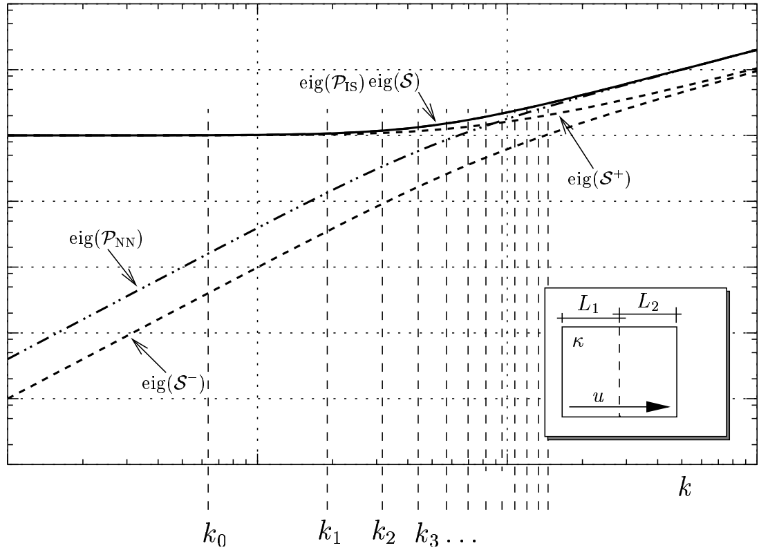
Fig. 7. Eigenvalues of Steklov operators and preconditioners for the advection-diffusion operator ( \text{Pe} = 50 ) and symmetric partitions ( L_1 = L_2 = L/2 , b = 0.1L ).
