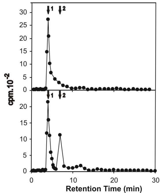
Figure 1. HPLC analysis of in vivo induction of NBAD synthesis. Non-sclerotizing T. molitor larvae V were injected with a micro-needle. Injections of 13 \mu l insect ringer contained [ 14 C] \beta -alanine as substrate tracer without bacteria (upper panel) or with bacteria (lower panel). Arrows indicate the retention time of internal standards of \beta -alanine (1) and NBAD (2).
