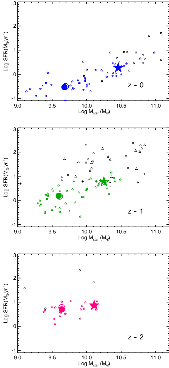
Figure 3. Mean star formation rate as a function of the mean stellar mass of simulated galaxies in the low (large filled circles) and high (large filled stars) stellar-mass subsamples for z \sim 0 (blue symbols; upper panel), z \sim 1 (green symbols; middle panel), z \sim 2 (magenta symbols; lower panel). Small open stars represent the values for individual simulated galaxies. Mean estimations obtained by excluding galaxies with slopes < -0.1 \text{ dex kpc}^{-1} are also included (open symbols). Most of them are superposed to the mean values from the whole sample. For comparison, we included the observational results from Rupke et al. (2010) , (black squares; z \sim 0 ), Queyrel et al. (2012) , (black triangles; z \sim 1 ), Stott et al. (2014) , (black, crosses; z \sim 1 ) and Jones et al. (2013) , (black, diamonds; z \sim 2 ). Mean values and error bars were estimated by applying a bootstrap technique.
