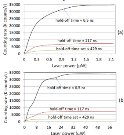
Fig. 9 Photon counting rates measured for different incident laser powers.
