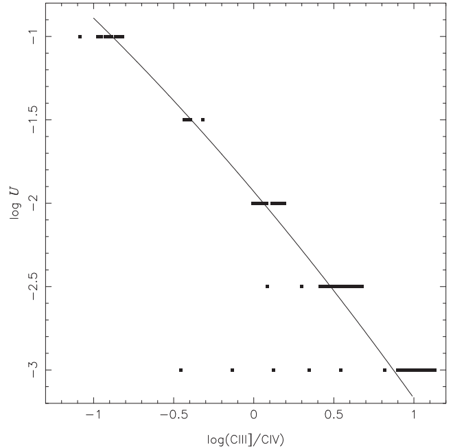
Figure 5. Logarithm of the ionization parameter versus \log(C\text{III}/C\text{IV}) . The points represent the results from our models considering different values for Z and \log U . The curve represents a fitting (equation 1) to the average points for each \log U value.
