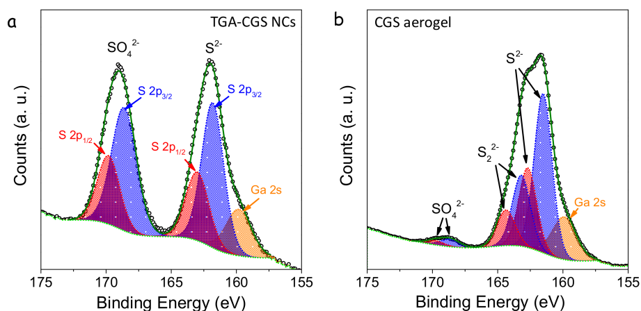
Figure 6. S 2p region of the XPS spectra of the TGA-CGS NCs (a) and the CGS NC-based aerogel (b). S 2p 3/2 states are plotted in blue and S 2p 1/2 states in red. In the same region, the Ga 2s state is observed.
