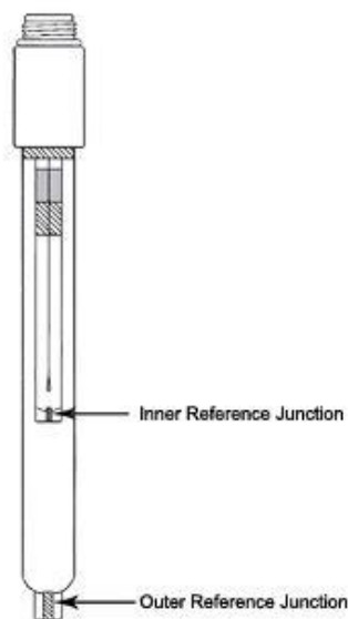
Double Junction Reference Electrode
