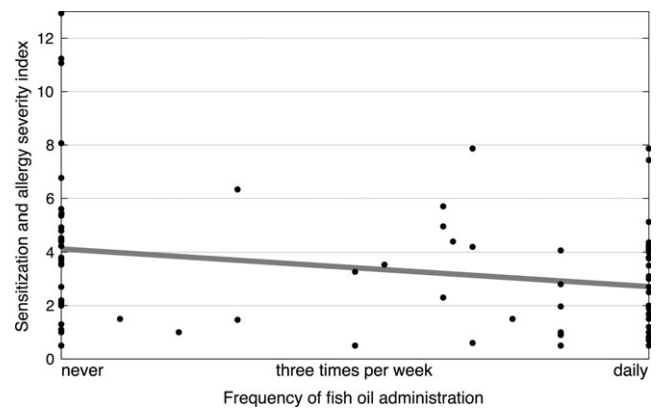
FIGURE 2 Sensitization and allergy severity index according to the frequency of fish oil administration. There was a significant relationship (linear regression t test, P = .013 )
