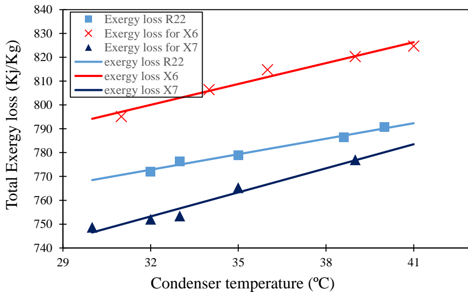
Figure 9. Exergy loss developing with condenser temperature.
