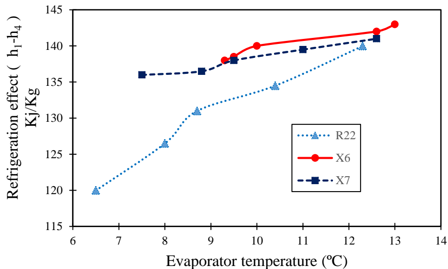
Figure 6. Change in refrigerating effect with respect to evaporator temperature.
