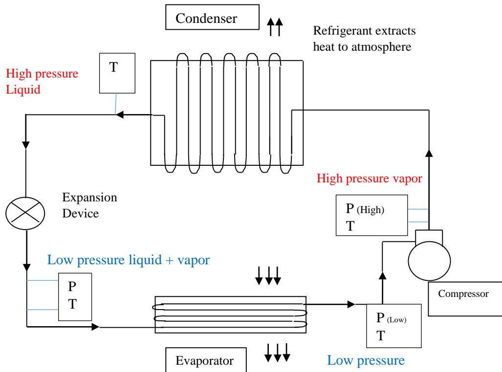
Figure 1. Schematic diagram of experimental setup.
