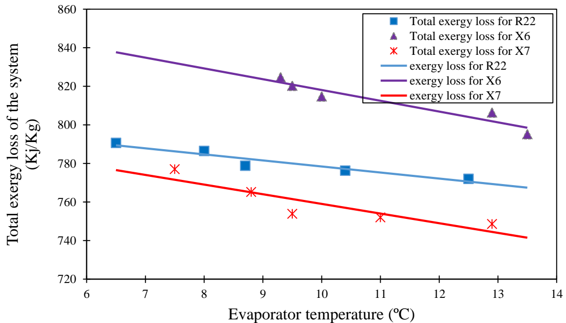
Figure 8. Change in exergy loss with evaporator temperature.
