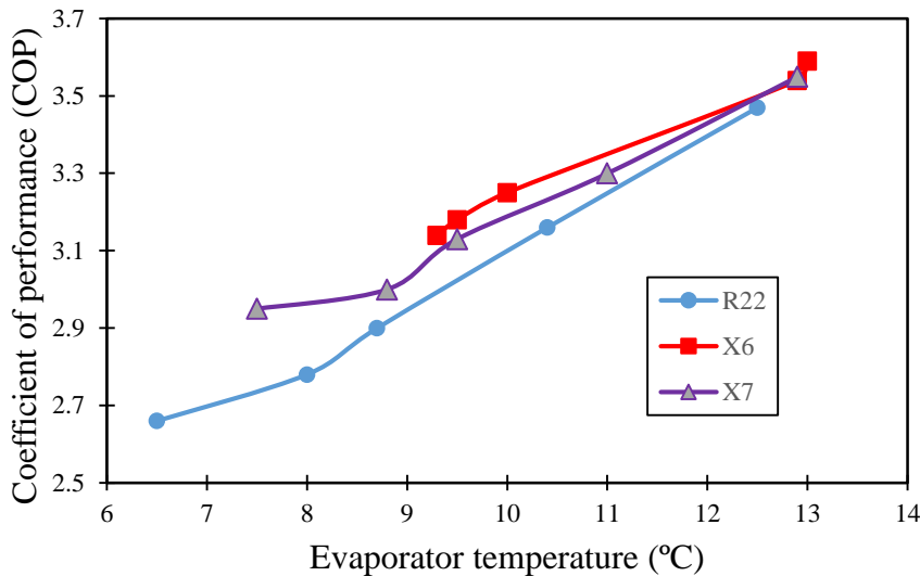
Figure 5. Change in COP with evaporator temperature.
