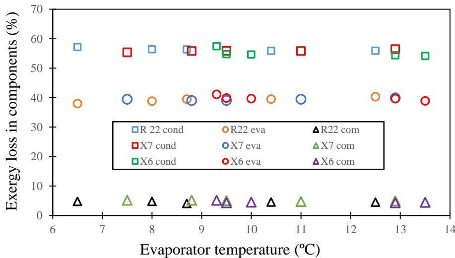
Figure 10. Percentage exergy loss in various components with evaporator temperature.
