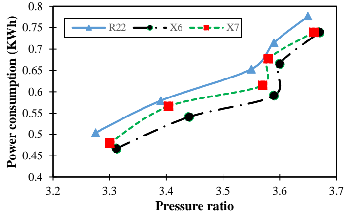
Figure 7. Relationship between power consumption and pressure ratio.
