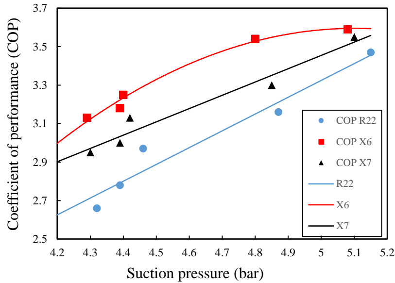
Figure 4. Variation in COP with evaporator pressure.
