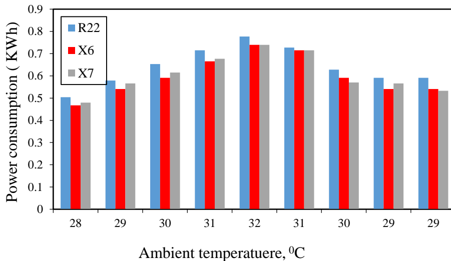
Figure 3. Variations of power consumptions using R22, X 6 and X 7 at different ambient temperatures.
