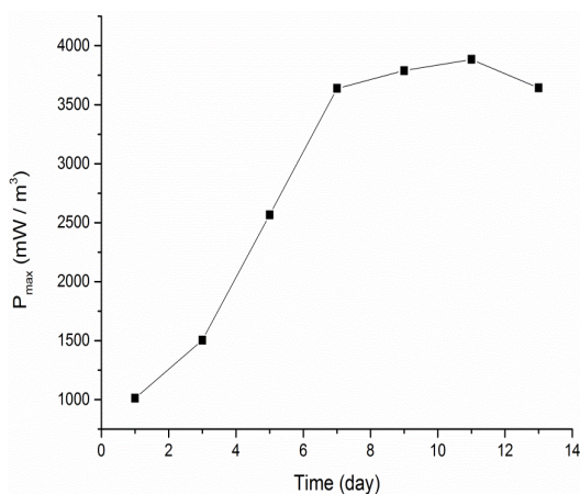
Fig. 1: Maximum power densities of the MFC versus time.
