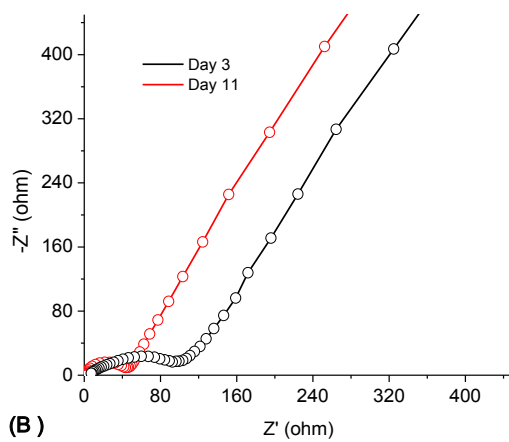
Fig. 4: Nyquist plots of B. cereus on the 3 rd and 11 th day of operations.
