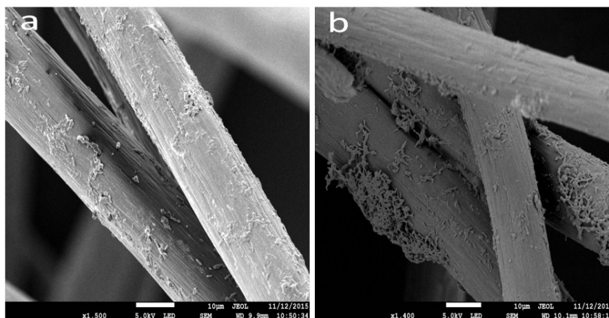
Fig. 3: FESEM images on anode carbon brush in the MFC fed with POME as substrate, (a) day 3 and (b) day 11.
