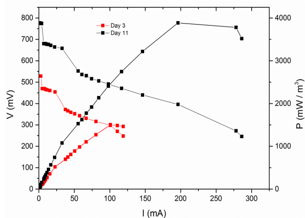
Fig. 2: Polarization curves of the MFC on the 3 rd and 11 th day using B. cereus .
