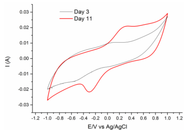
Fig. 5: Cyclic voltammetry curves of B. cereus on the 3 rd day and 11 th day of operations.
