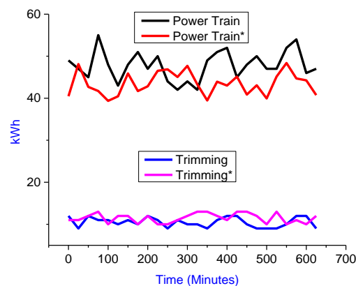
Figure 12. Power Train assembly and Trimming energy usage
